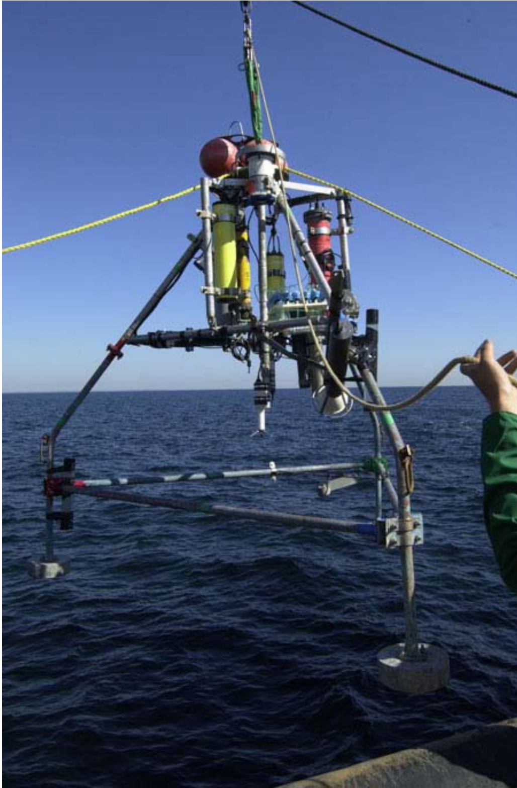
Figure 3. Tripod frame being deployed from USCG Cutter Marcus Hannah .
