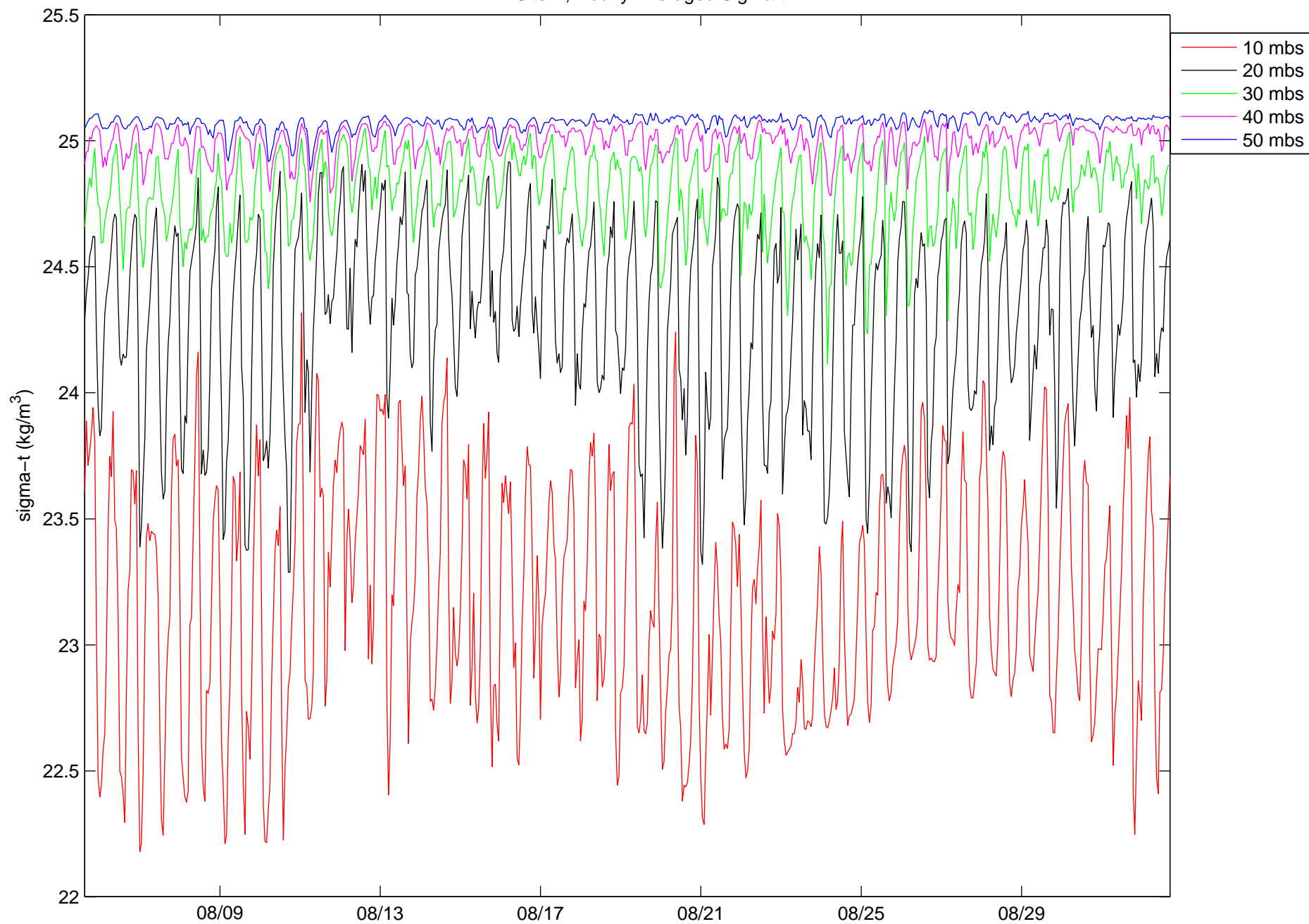
Site A, Hourly Averaged Sigma-t
