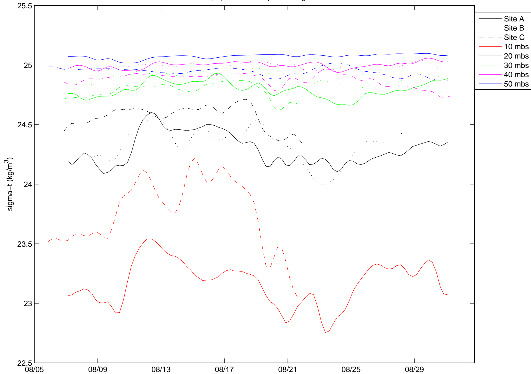
Sites A, B, and C: Low-passed Sigma-t
