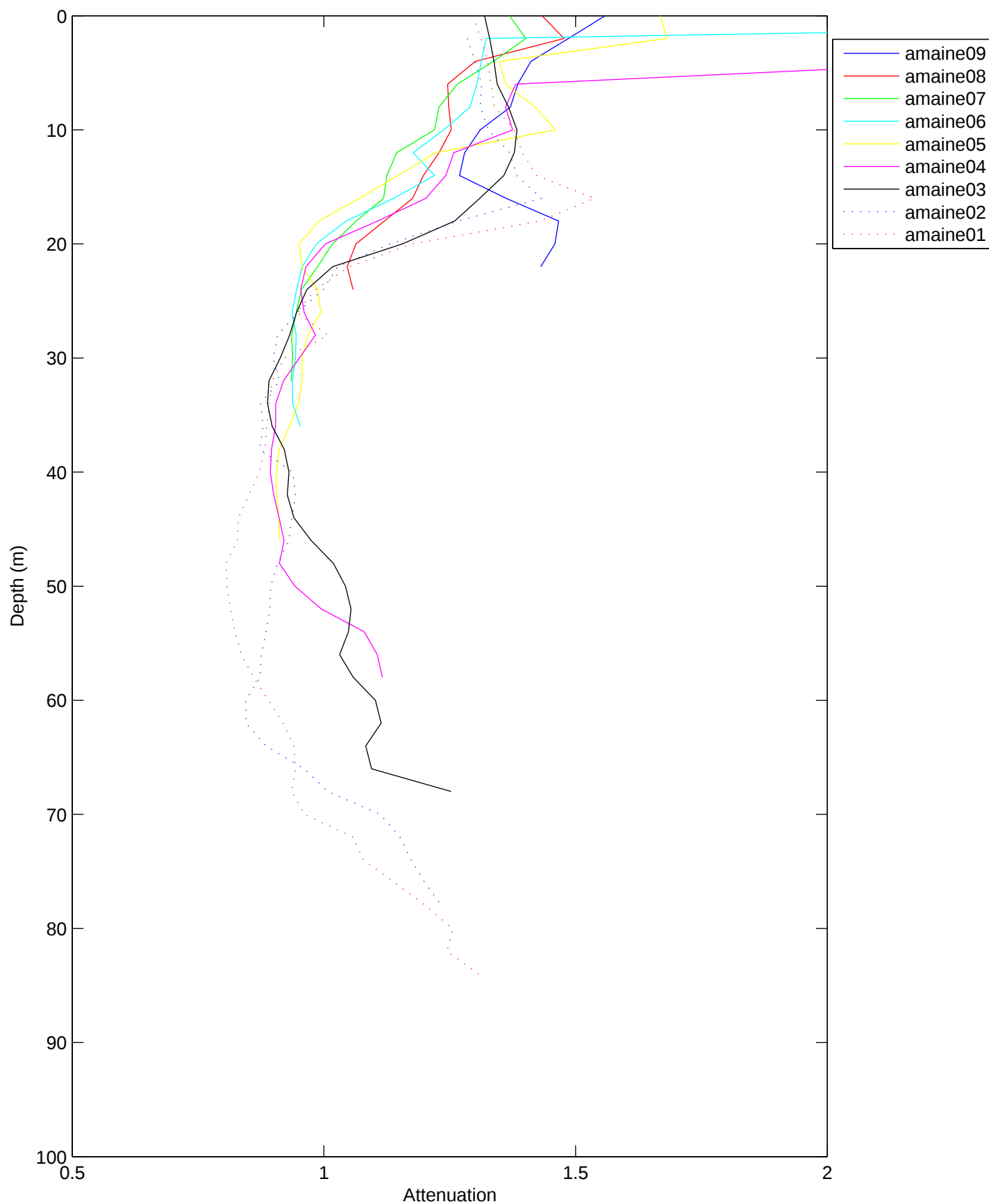
Attenuation, Argo Maine Transect 1: 31-Aug-1998 06:08 to 31-Aug-2004 11:17 01:48 after low water to 06:57 after low water
