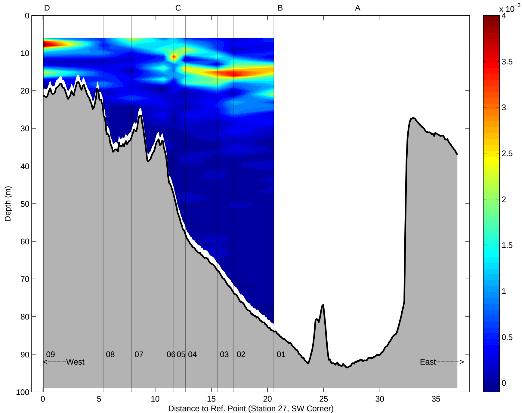
Brunt-Vaisala Frequency, Argo Maine Transect 1: 31-Aug-1998 06:08 to 31-Aug-2006 11:17 01:48 after low water to 06:57 after low water
