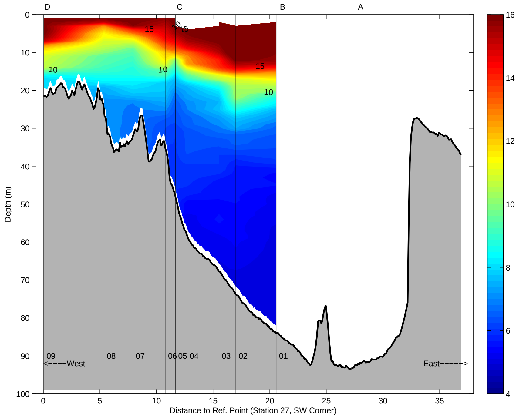
Temperature, Argo Maine Transect 1: 31-Aug-1998 06:08 to 31-Aug-2006 11:17 01:48 after low water to 06:57 after low water
