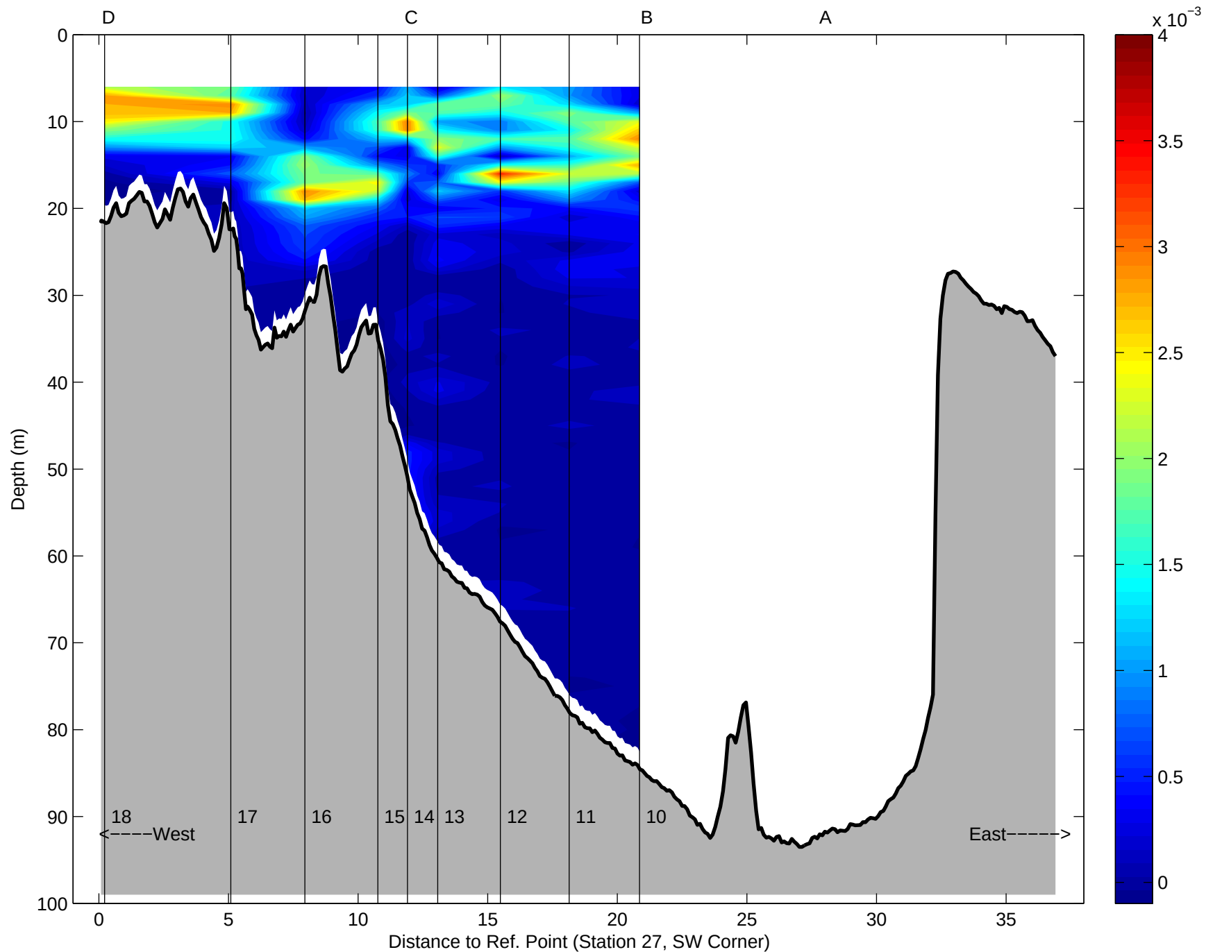
Brunt-Vaisala Frequency, Argo Maine Transect 2: 31-Aug-1998 15:06 to 31-Aug-1998 17:29 10:46 after low water to 13:09 after low water
