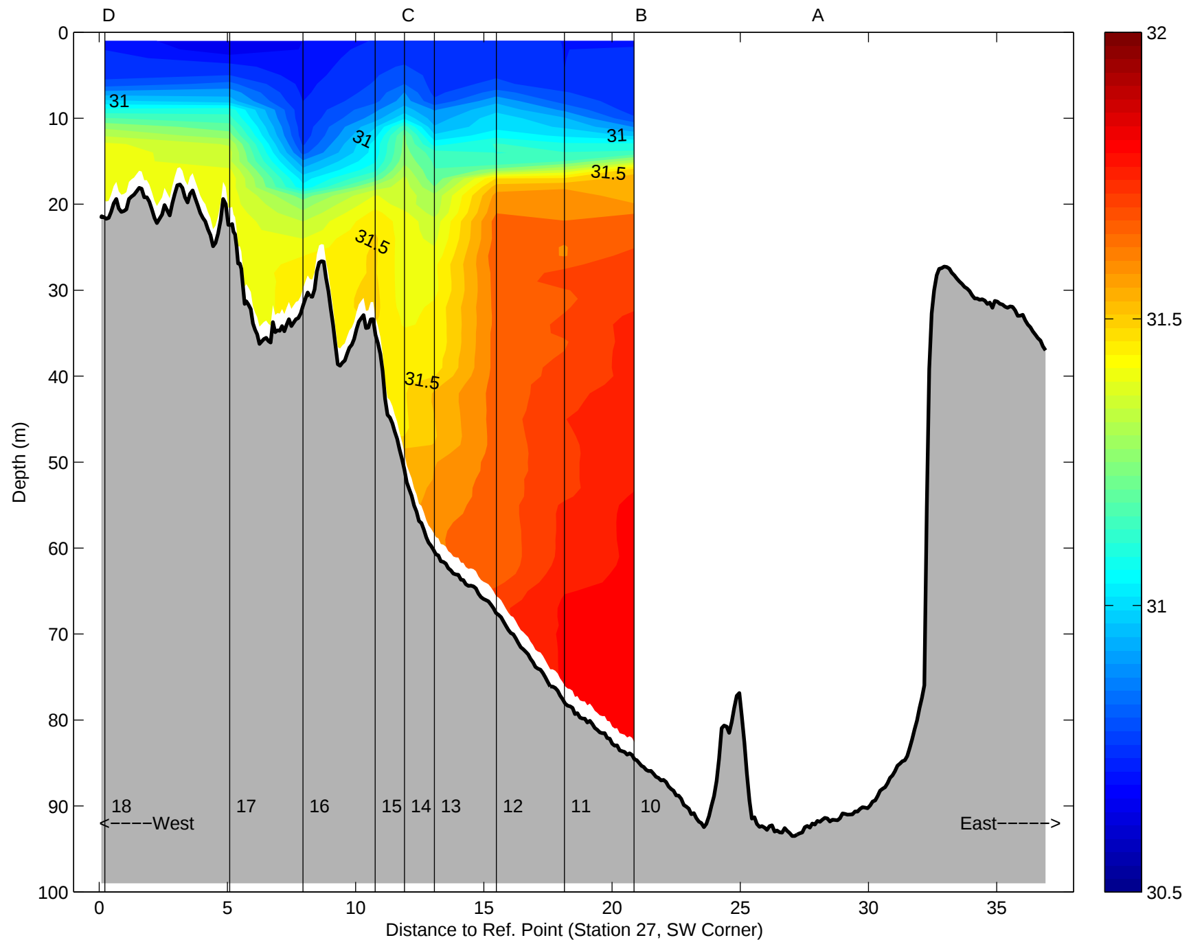
Salinity, Argo Maine Transect 2: 31-Aug-1998 15:06 to 31-Aug-1998 17:29 10:46 after low water to 13:09 after low water
