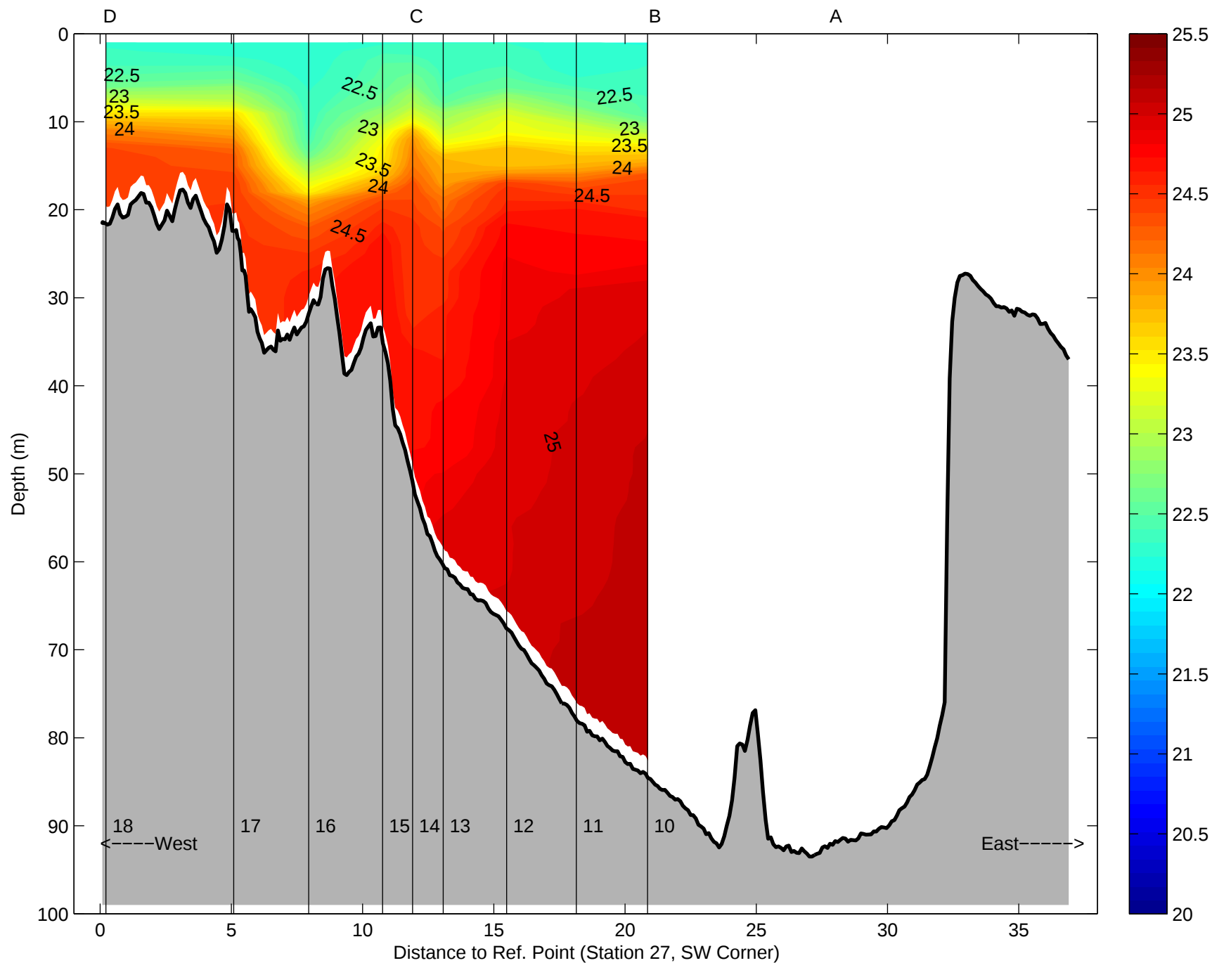
Sigma Theta, Argo Maine Transect 2: 31-Aug-1998 15:06 to 31-Aug-1998 17:29 10:46 after low water to 13:09 after low water
