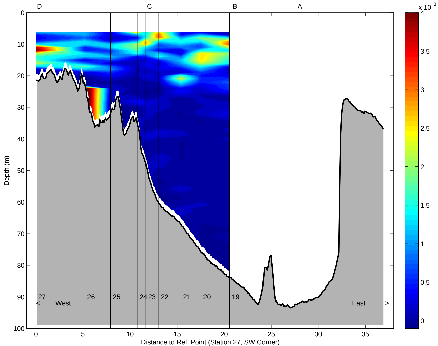
Brunt-Vaisala Frequency, Argo Maine Transect 3: 31-Aug-1998 18:49 to 31-Aug-1998 21:05 02:15 after low water to 04:31 after low water
