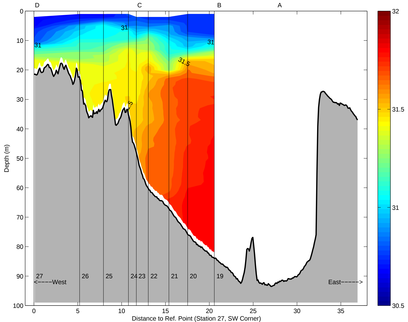
Salinity, Argo Maine Transect 3: 31-Aug-1998 18:49 to 31-Aug-1998 21:05 02:15 after low water to 04:31 after low water
