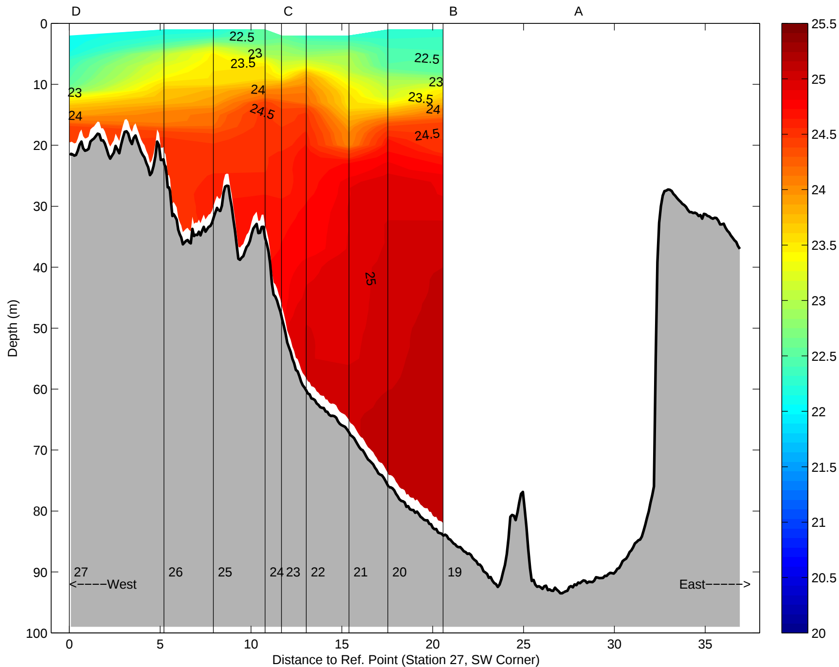
Sigma Theta, Argo Maine Transect 3: 31-Aug-1998 18:49 to 31-Aug-1998 21:05 02:15 after low water to 04:31 after low water
