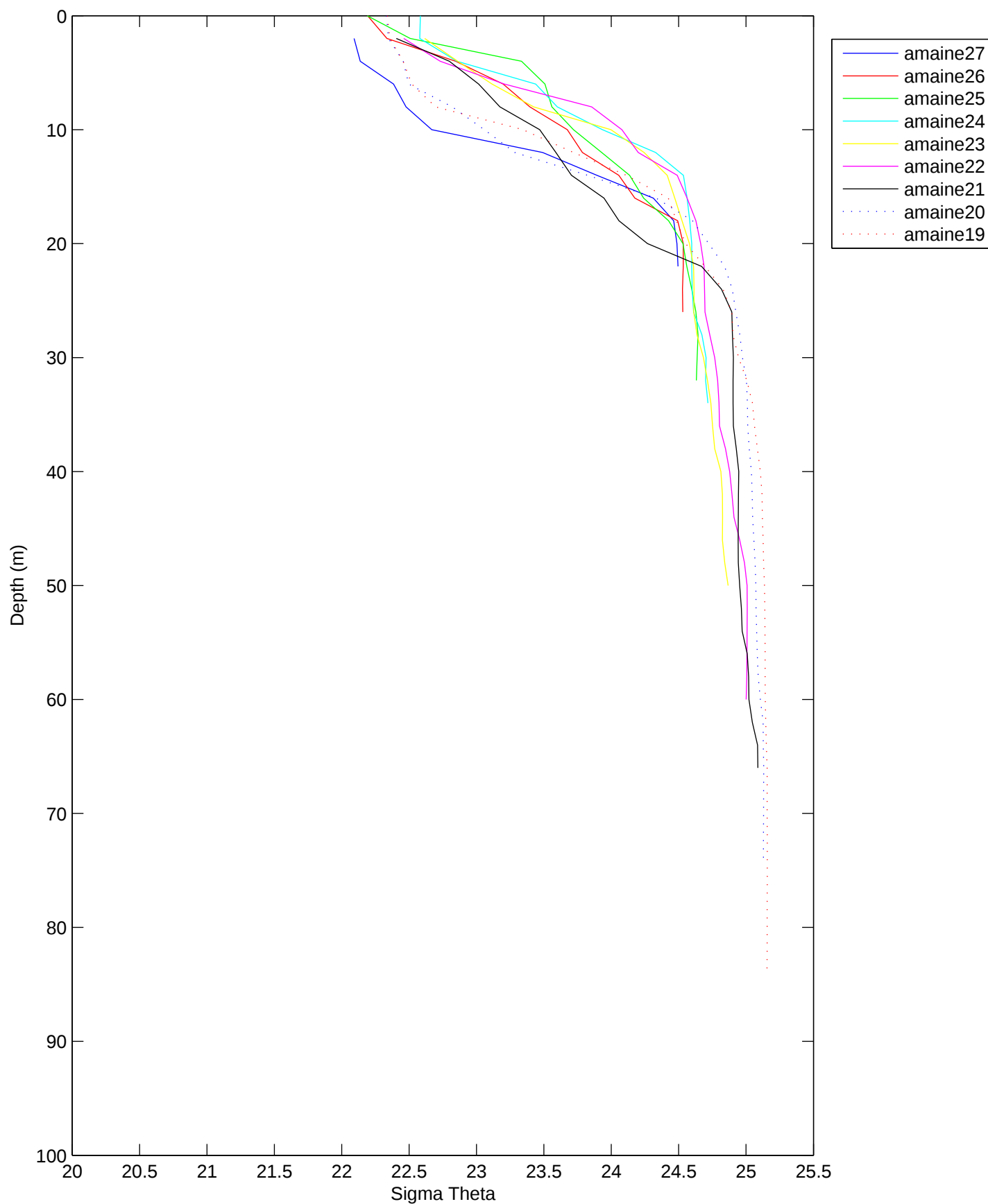
Sigma Theta, Argo Maine Transect 3: 31-Aug-1998 18:49 to 31-Aug-1998 21:05 02:15 after low water to 04:31 after low water
