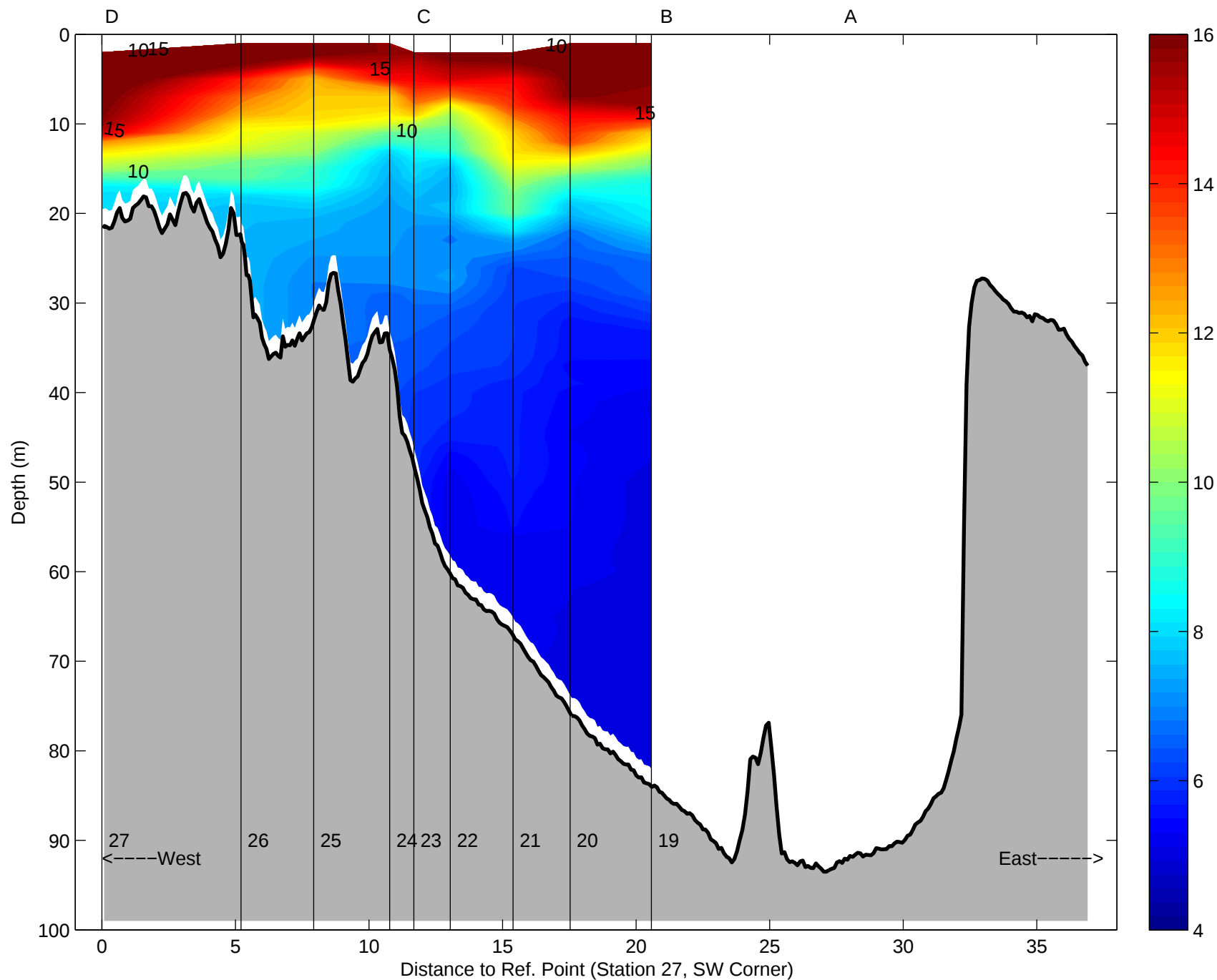
Temperature, Argo Maine Transect 3: 31-Aug-1998 18:49 to 31-Aug-1998 21:05 02:15 after low water to 04:31 after low water
