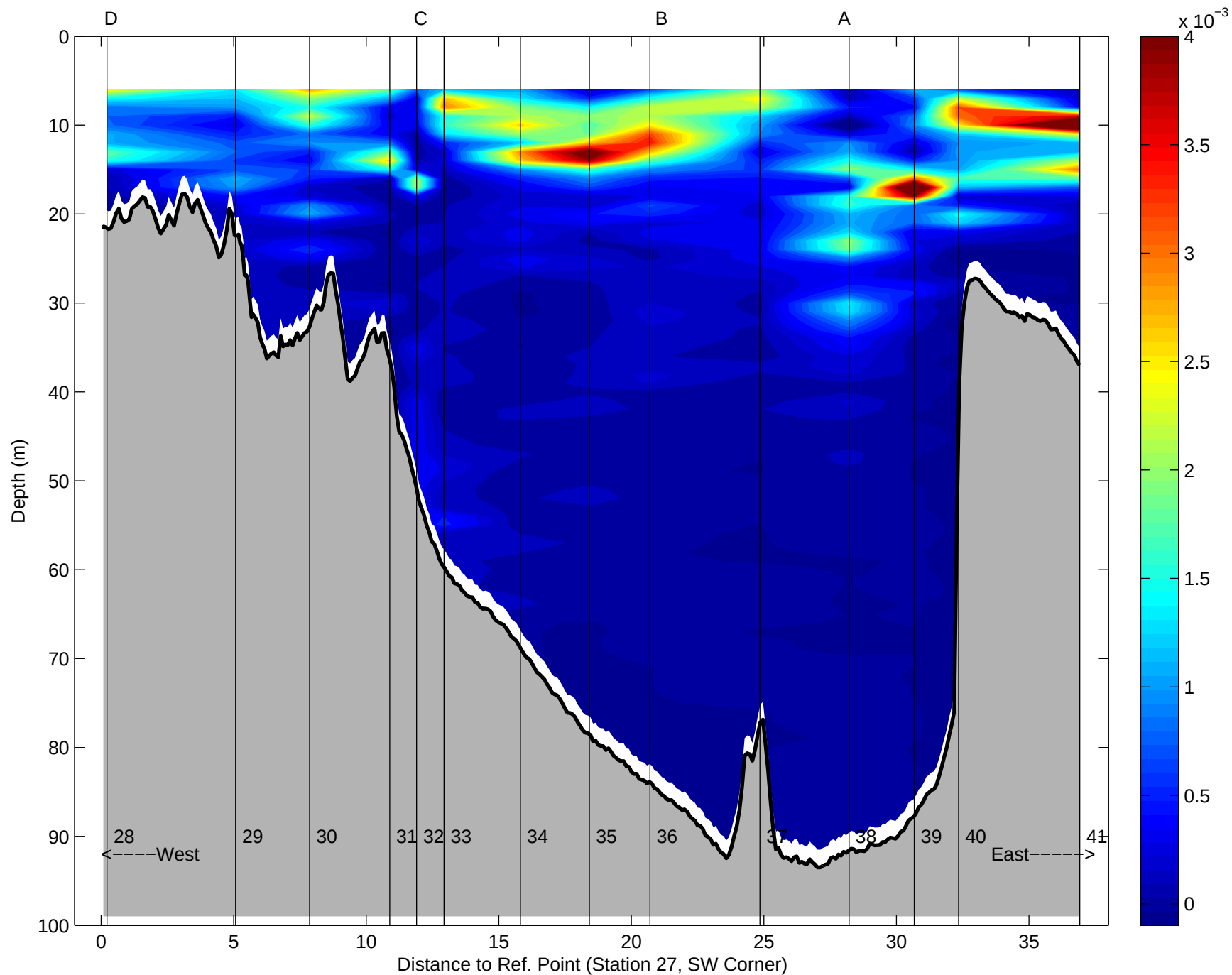
Brunt-Vaisala Frequency, Argo Maine Transect 4: 01-Sep-1998 04:20 to 01-Sep-1998 08:22 11:46 after low water to 15:48 after low water
