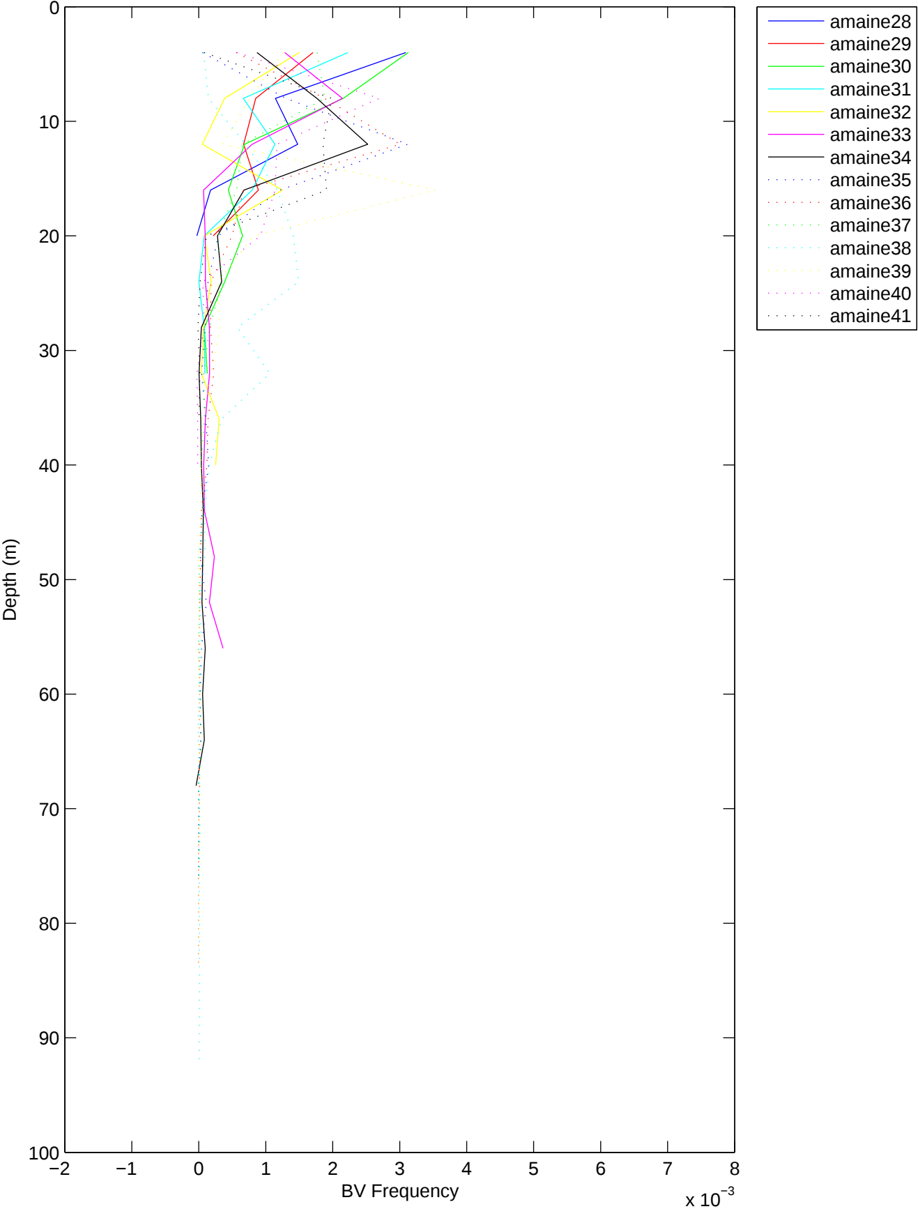
Brunt-Vaisala Frequency, Argo Maine Transect 4: 01-Sep-1998 04:20 to 01-Sep-1998 08:22 11:46 after low water to 15:48 after low water
