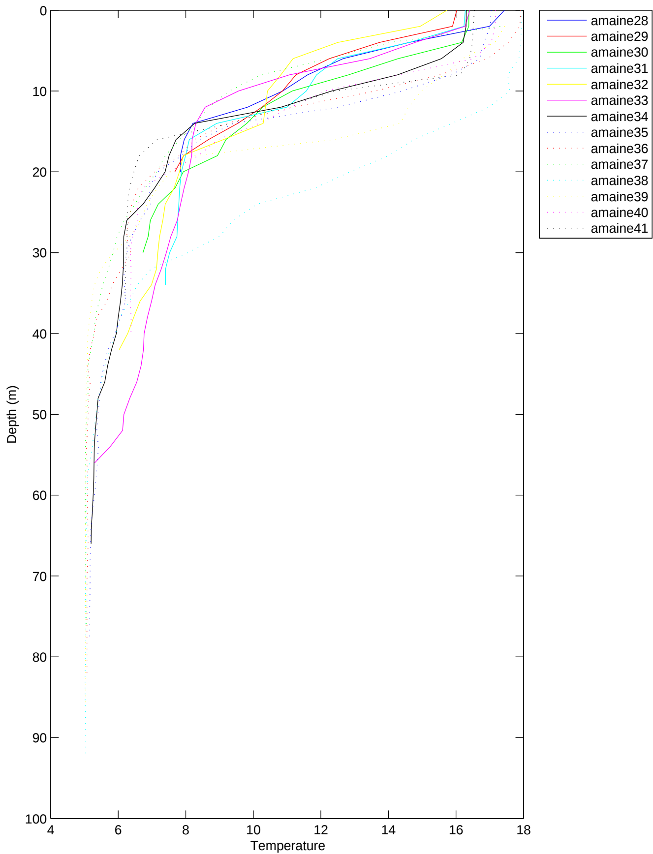
Temperature, Argo Maine Transect 4: 01-Sep-1998 04:20 to 01-Sep-1998 08:22 11:46 after low water to 15:48 after low water
