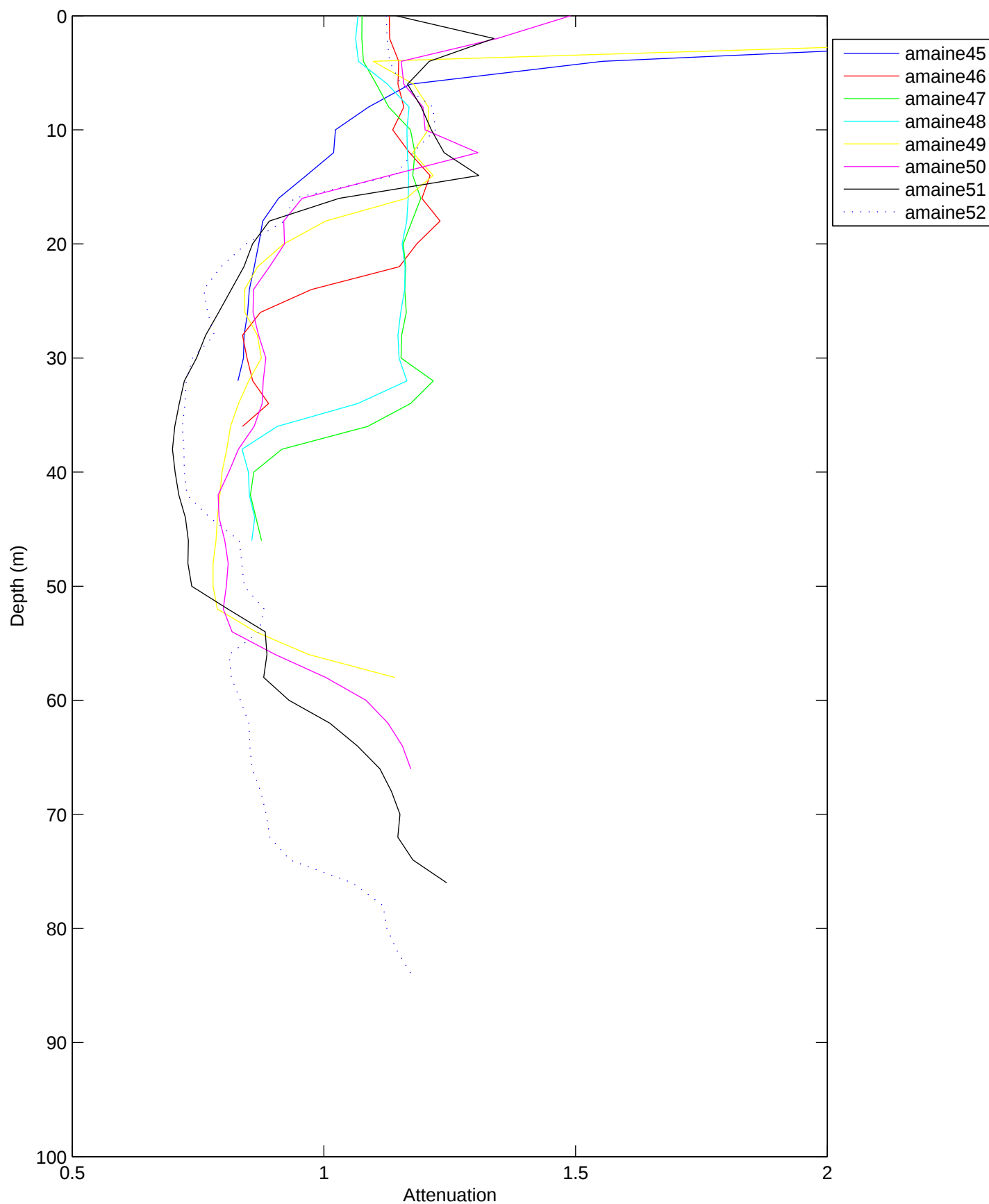
Attenuation, Argo Maine Transect 5: 02-Sep-1998 03:41 to 02-Sep-1998 05:32 10:17 after low water to 12:08 after low water
