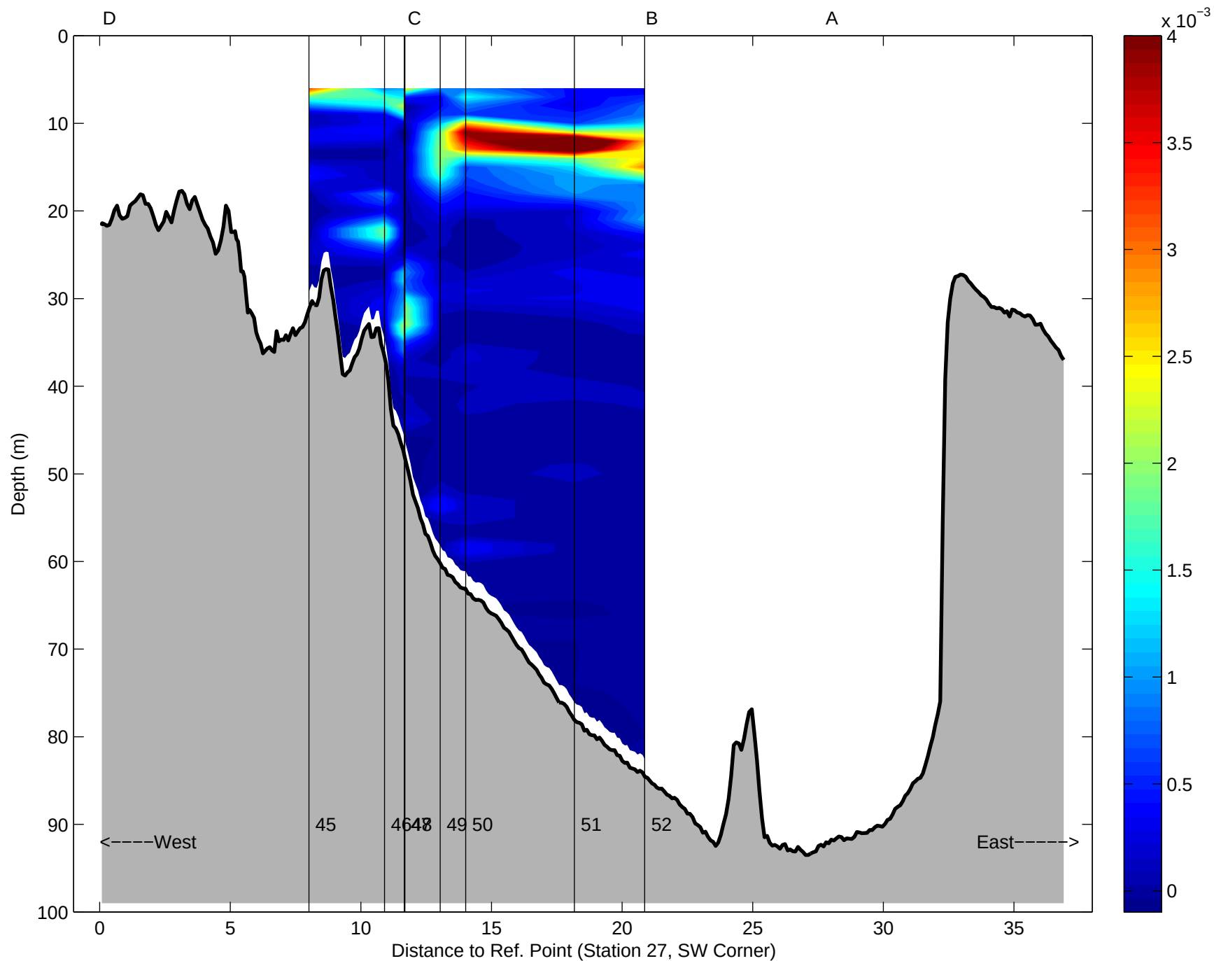
Brunt-Vaisala Frequency, Argo Maine Transect 5: 02-Sep-1998 03:41 to 02-Sep-1998 05:32 10:17 after low water to 12:08 after low water
