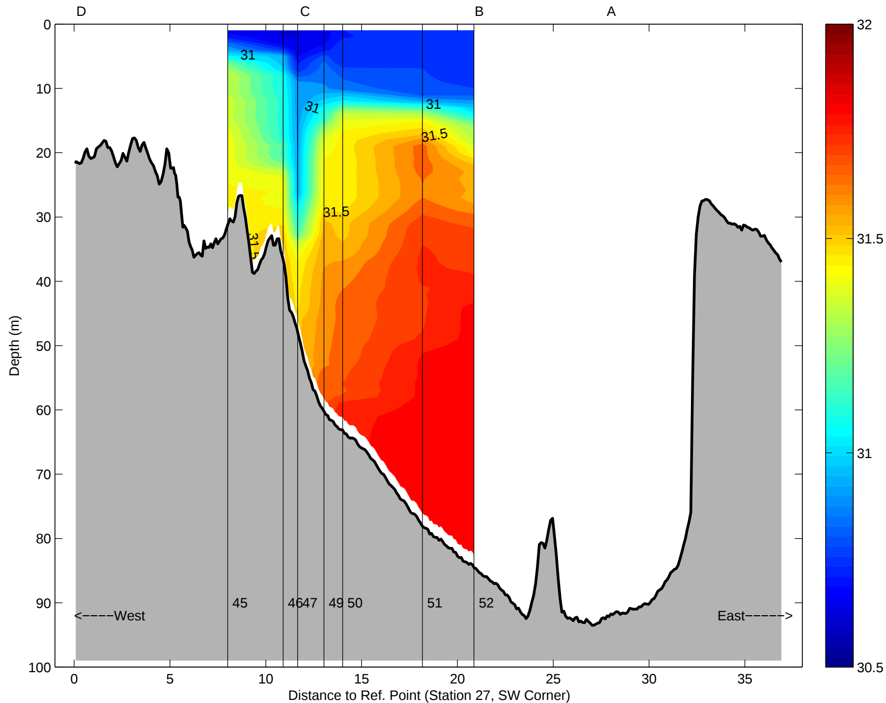
Salinity, Argo Maine Transect 5: 02-Sep-1998 03:41 to 02-Sep-1998 05:32 10:17 after low water to 12:08 after low water
