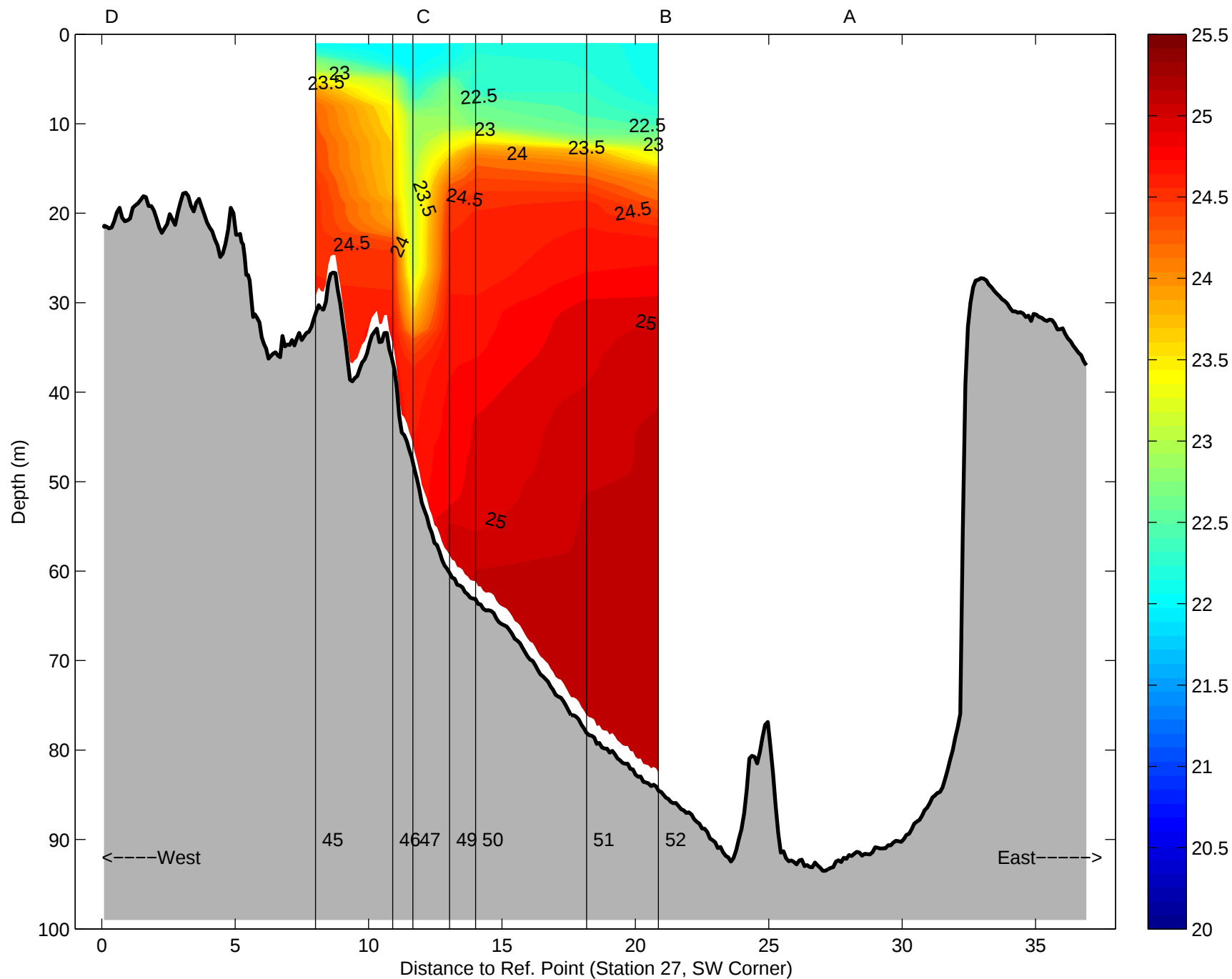
Sigma Theta, Argo Maine Transect 5: 02-Sep-1998 03:41 to 02-Sep-1998 05:32 10:17 after low water to 12:08 after low water
