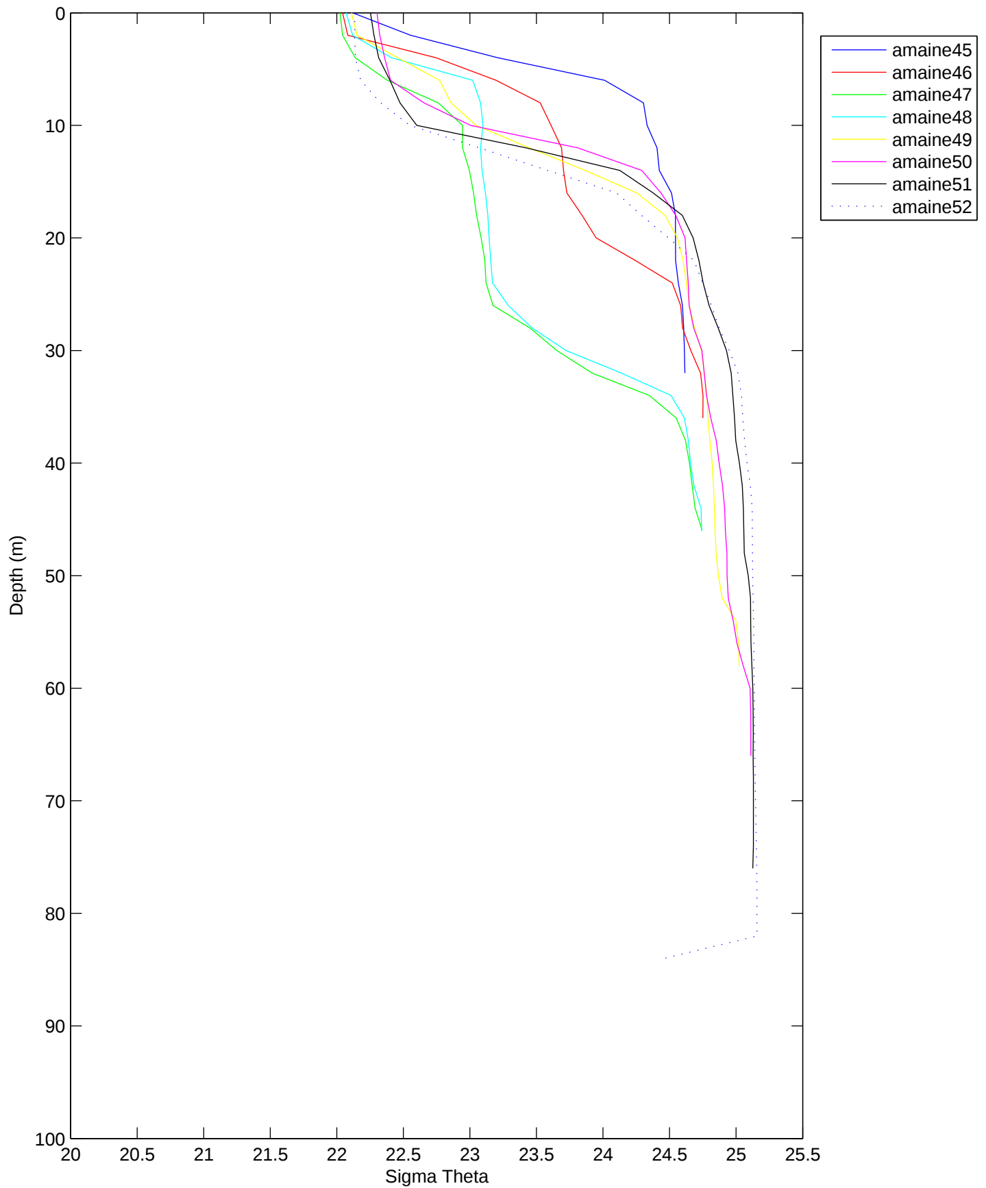
Sigma Theta, Argo Maine Transect 5: 02-Sep-1998 03:41 to 02-Sep-1998 05:32 10:17 after low water to 12:08 after low water
