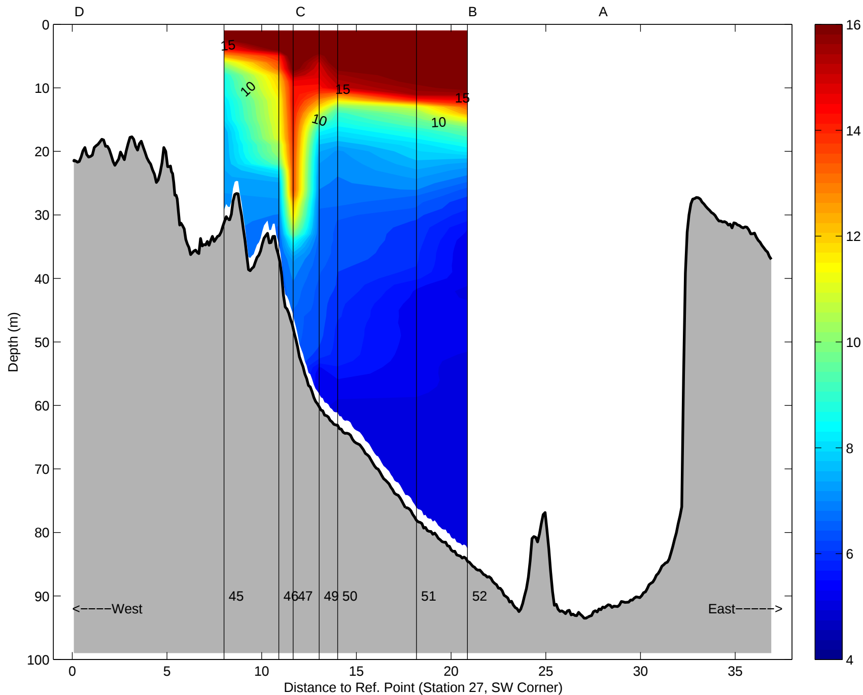
Temperature, Argo Maine Transect 5: 02-Sep-1998 03:41 to 02-Sep-1998 05:32 10:17 after low water to 12:08 after low water
