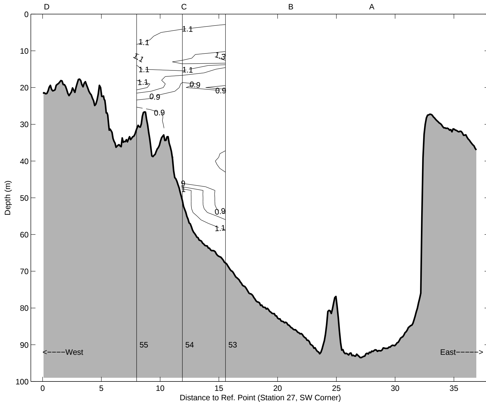
Attenuation, Argo Maine Transect 6: 02-Sep-1998 06:02 to 02-Sep-1998 06:47 12:38 after low water to 13:23 after low water
