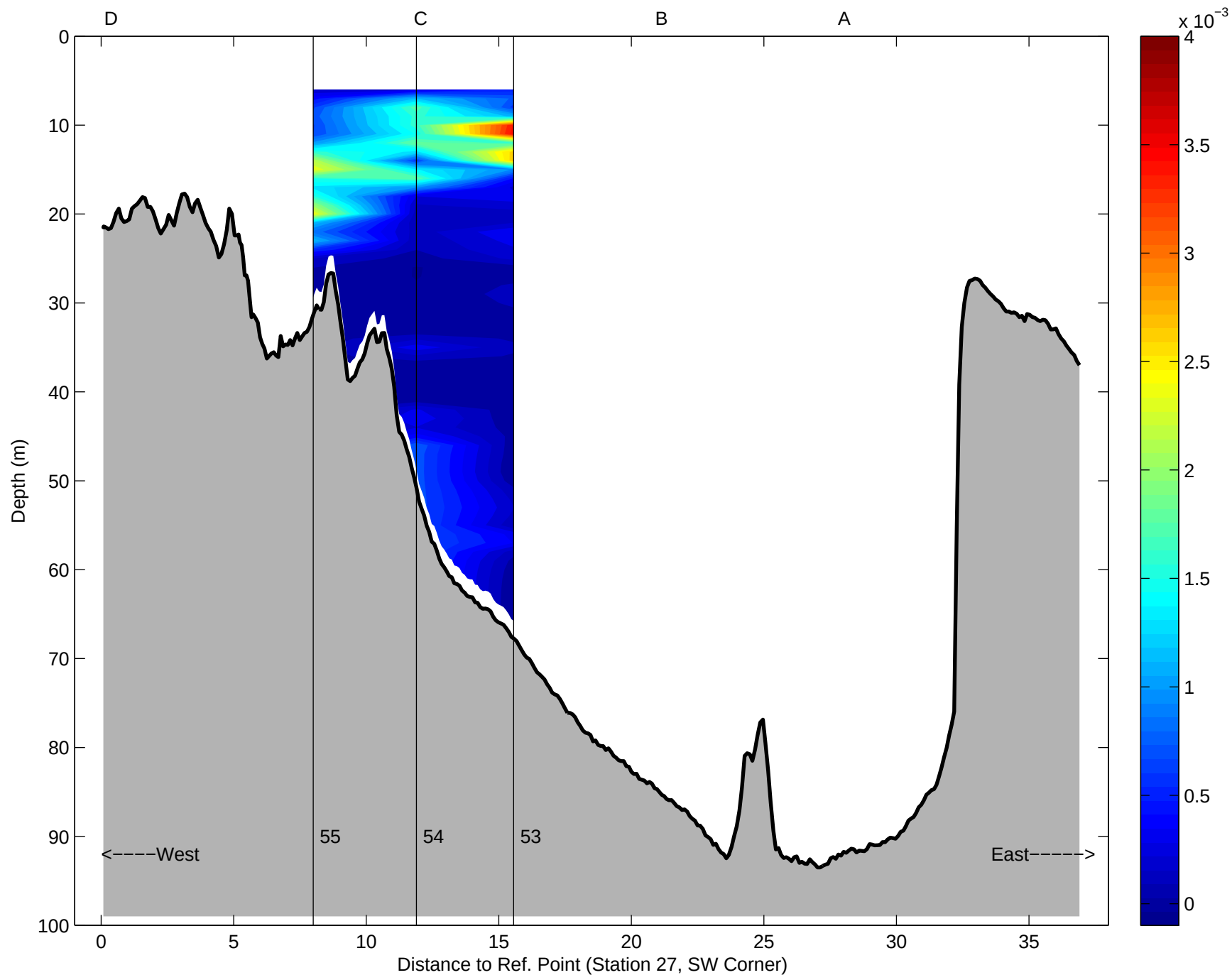
Brunt-Vaisala Frequency, Argo Maine Transect 6: 02-Sep-1998 06:02 to 02-Sep-1998 06:47 12:38 after low water to 13:23 after low water
