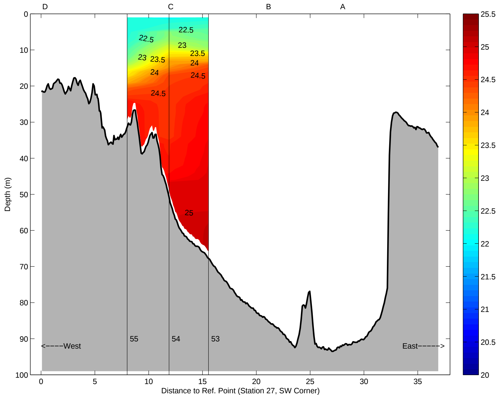
Sigma Theta, Argo Maine Transect 6: 02-Sep-1998 06:02 to 02-Sep-1998 06:47 12:38 after low water to 13:23 after low water
