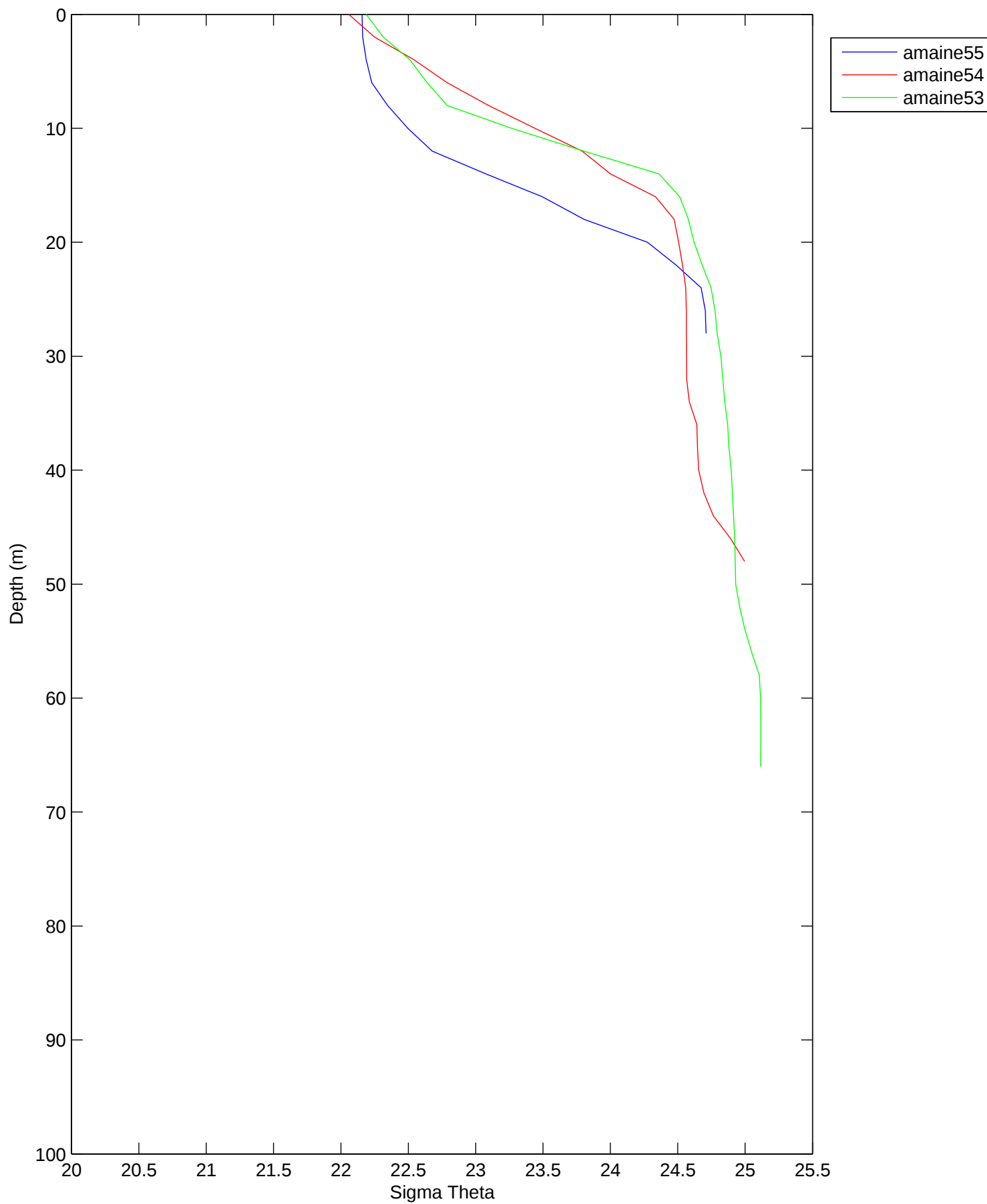
Sigma Theta, Argo Maine Transect 6: 02-Sep-1998 06:02 to 02-Sep-1998 06:47 12:38 after low water to 13:23 after low water
