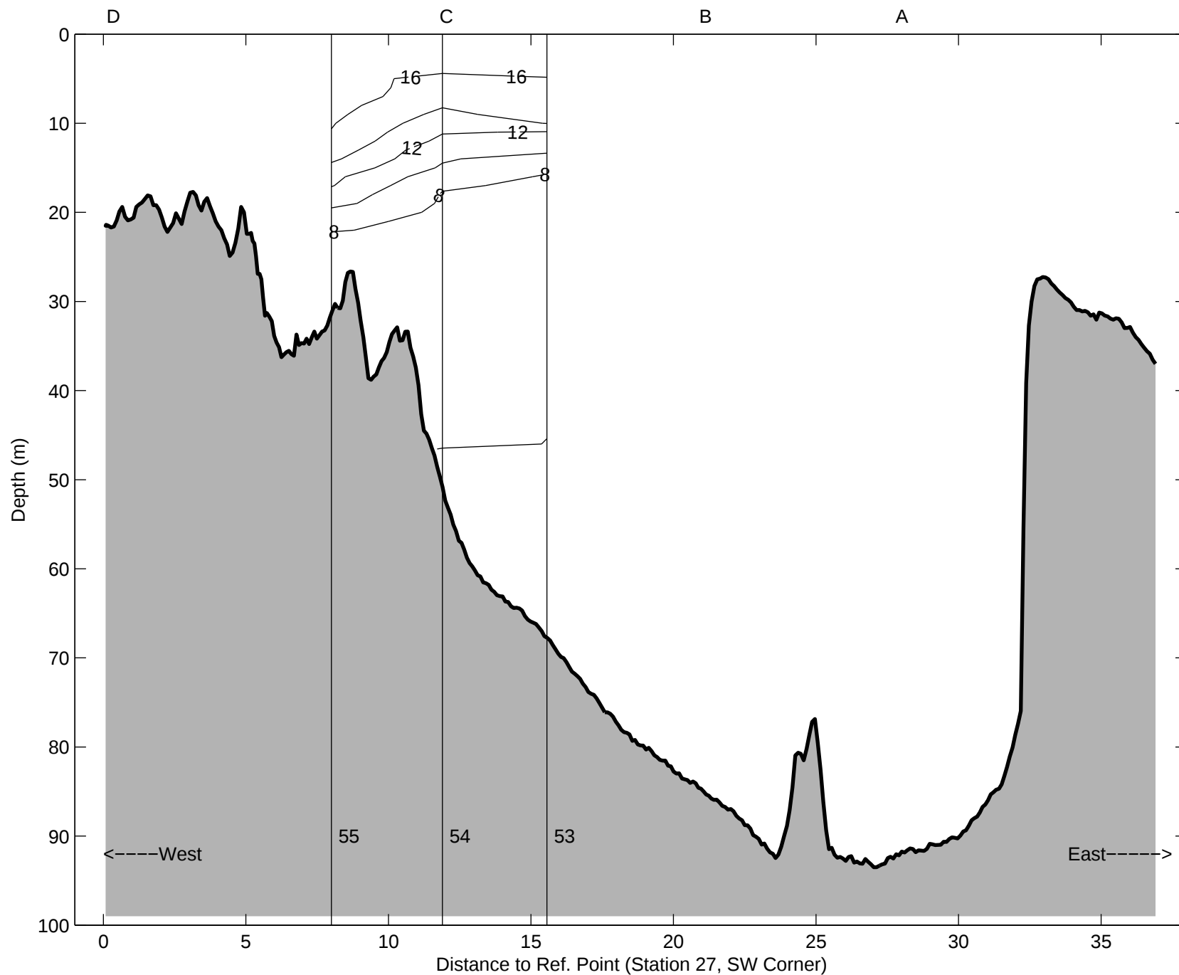
Temperature, Argo Maine Transect 6: 02-Sep-1998 06:02 to 02-Sep-1998 06:47 12:38 after low water to 13:23 after low water
