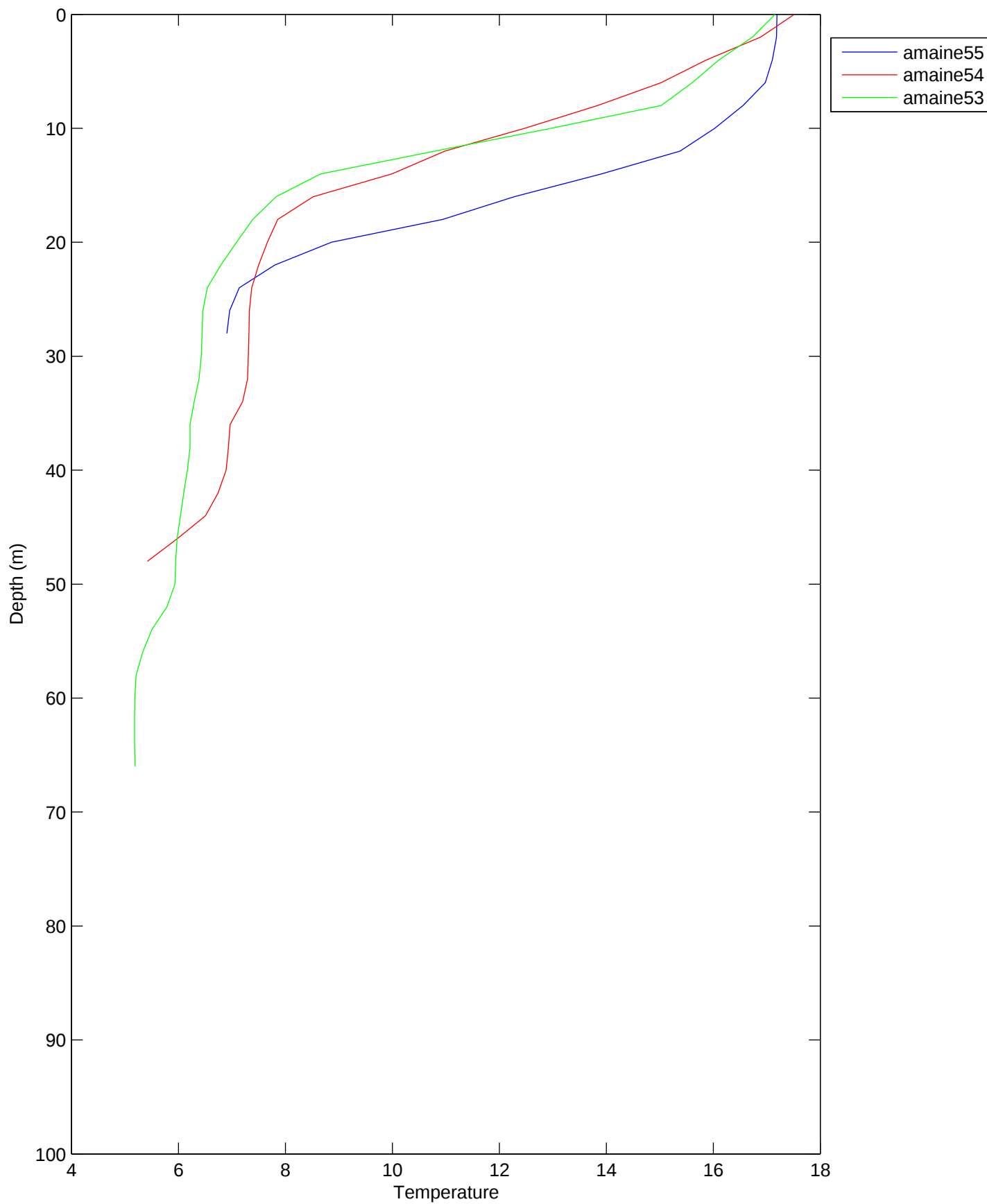
Temperature, Argo Maine Transect 6: 02-Sep-1998 06:02 to 02-Sep-1998 06:47 12:38 after low water to 13:23 after low water
