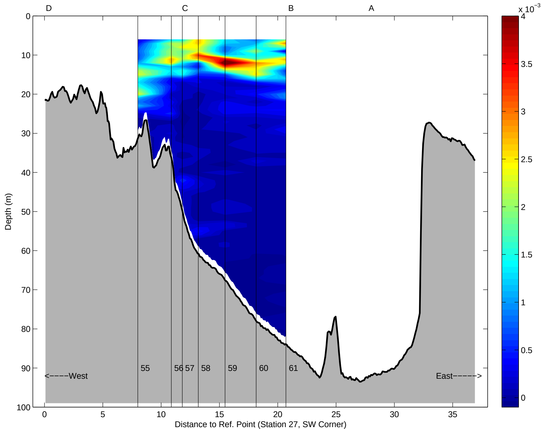
Brunt-Vaisala Frequency, Argo Maine Transect 7: 02-Sep-1998 06:47 to 02-Sep-1998 08:19 00:37 after low water to 02:09 after low water
