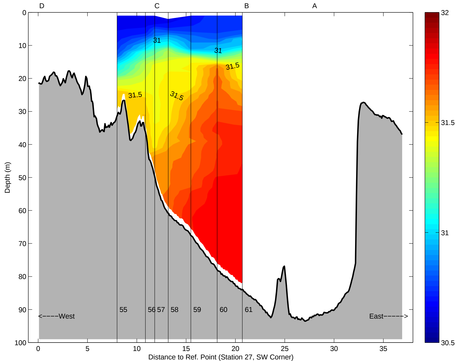
Salinity, Argo Maine Transect 7: 02-Sep-1998 06:47 to 02-Sep-1998 08:19 00:37 after low water to 02:09 after low water
