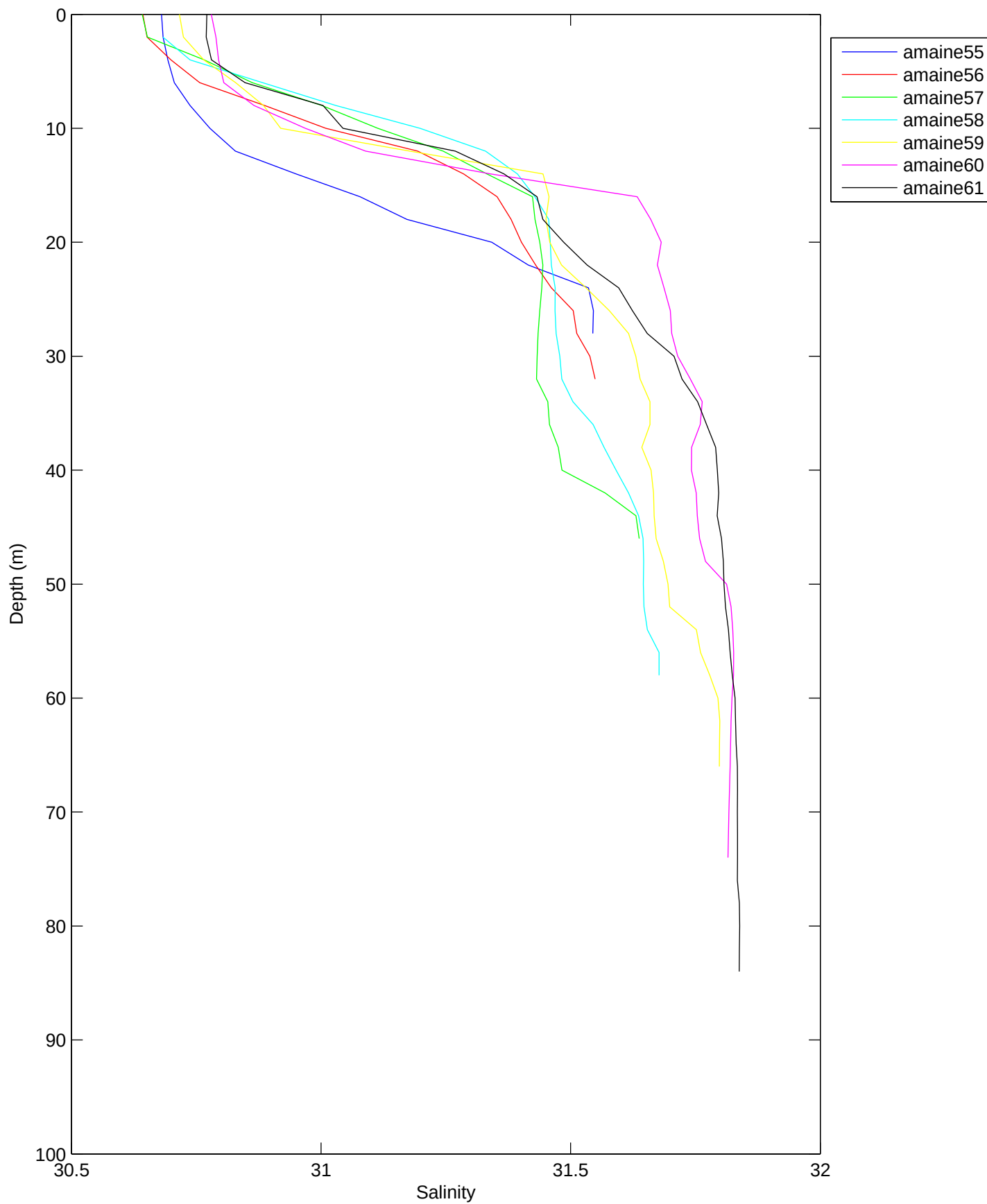
Salinity, Argo Maine Transect 7: 02-Sep-1998 06:47 to 02-Sep-1998 08:19 00:37 after low water to 02:09 after low water
