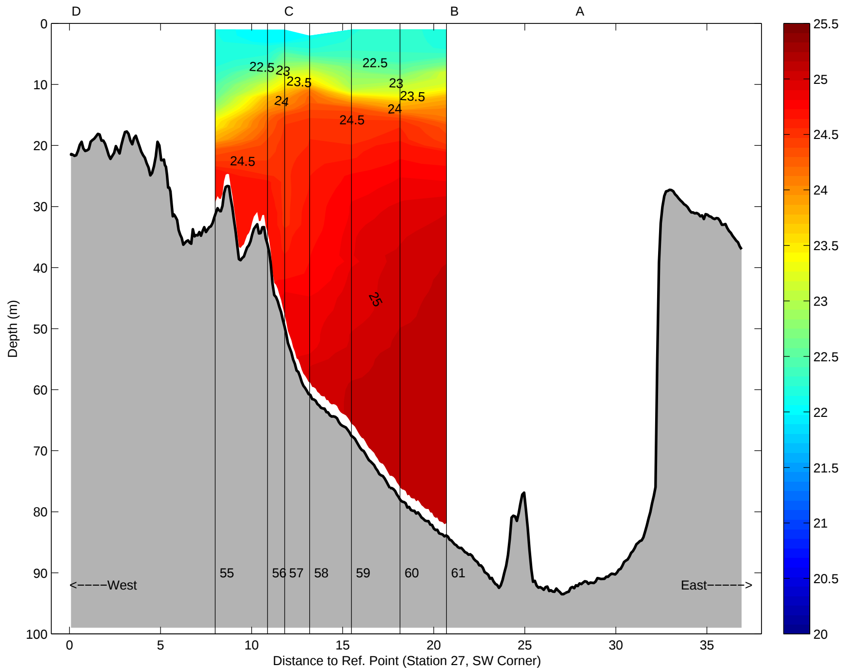
Sigma Theta, Argo Maine Transect 7: 02-Sep-1998 06:47 to 02-Sep-1998 08:19 00:37 after low water to 02:09 after low water
