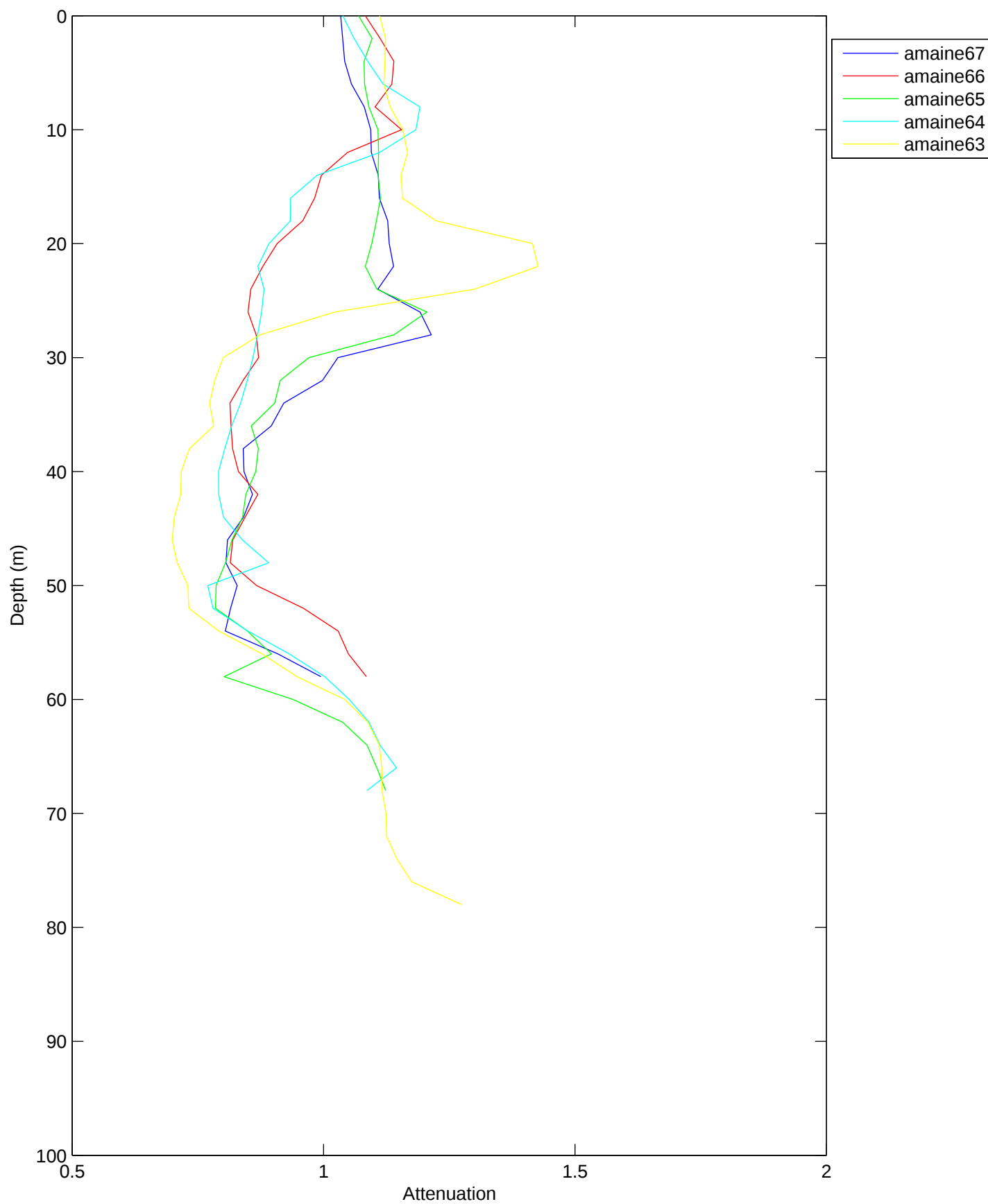
Attenuation, Argo Maine Transect 8: 02-Sep-1998 13:06 to 02-Sep-1998 15:24 06:56 after low water to 09:14 after low water
