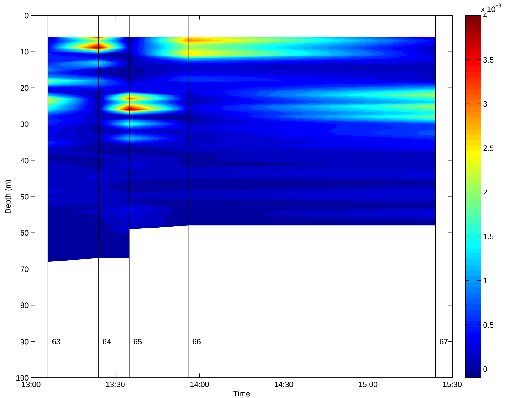
Brunt-Vaisala Frequency, Argo Maine Transect 8: 02-Sep-1998 13:06 to 02-Sep-1998 15:24 06:56 after low water to 09:14 after low water
