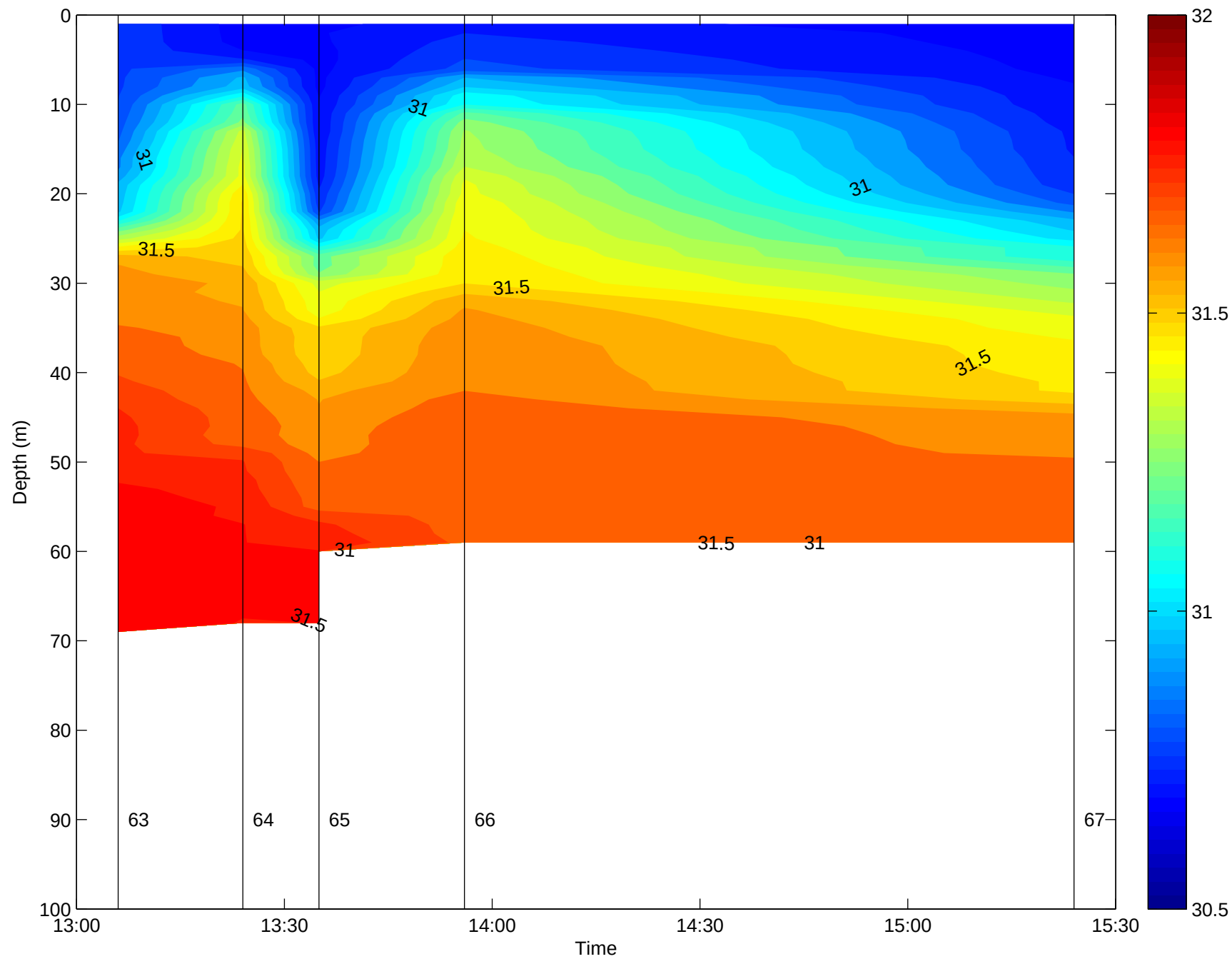
Salinity, Argo Maine Transect 8: 02-Sep-1998 13:06 to 02-Sep-1998 15:24 06:56 after low water to 09:14 after low water
