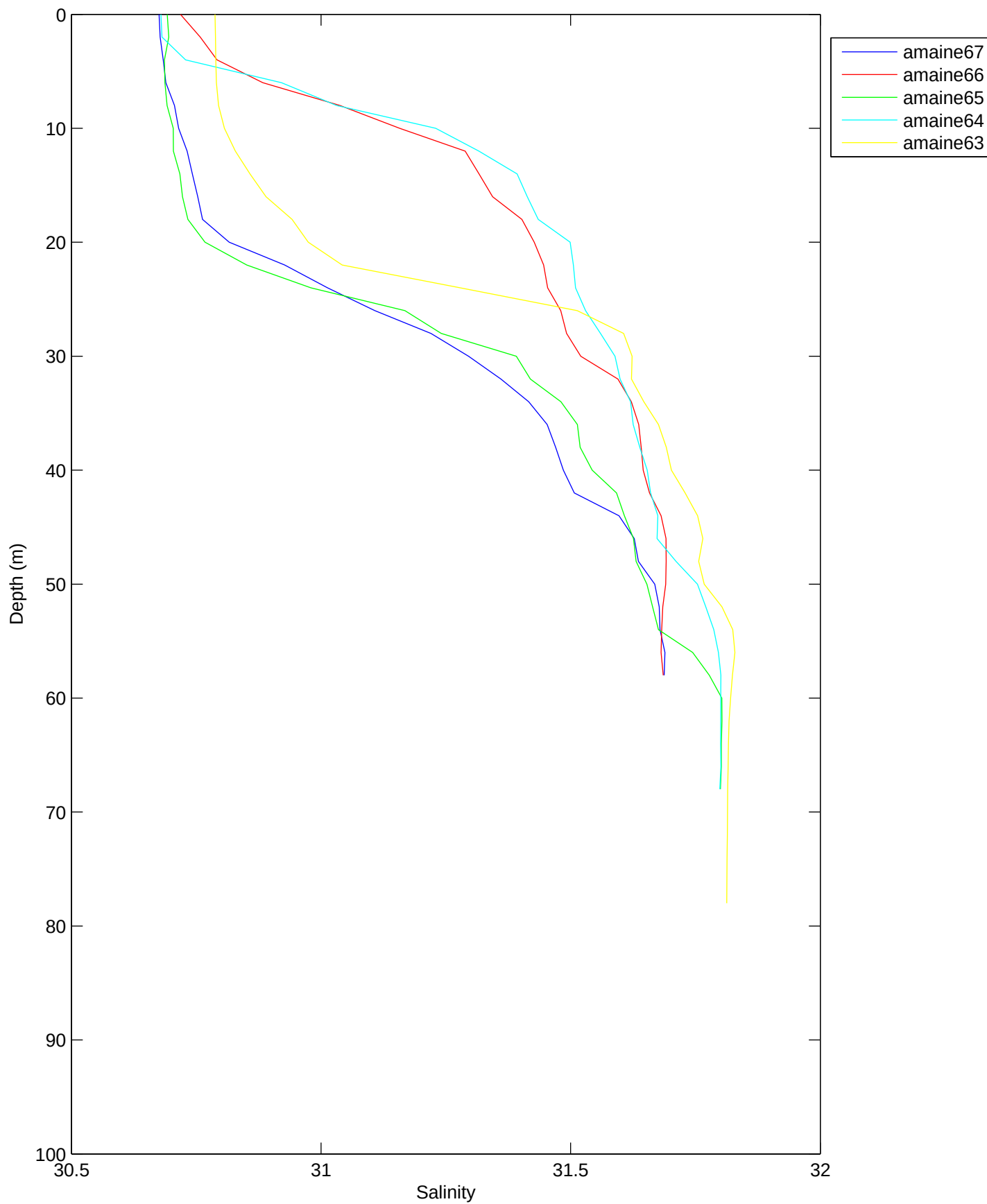
Salinity, Argo Maine Transect 8: 02-Sep-1998 13:06 to 02-Sep-1998 15:24 06:56 after low water to 09:14 after low water
