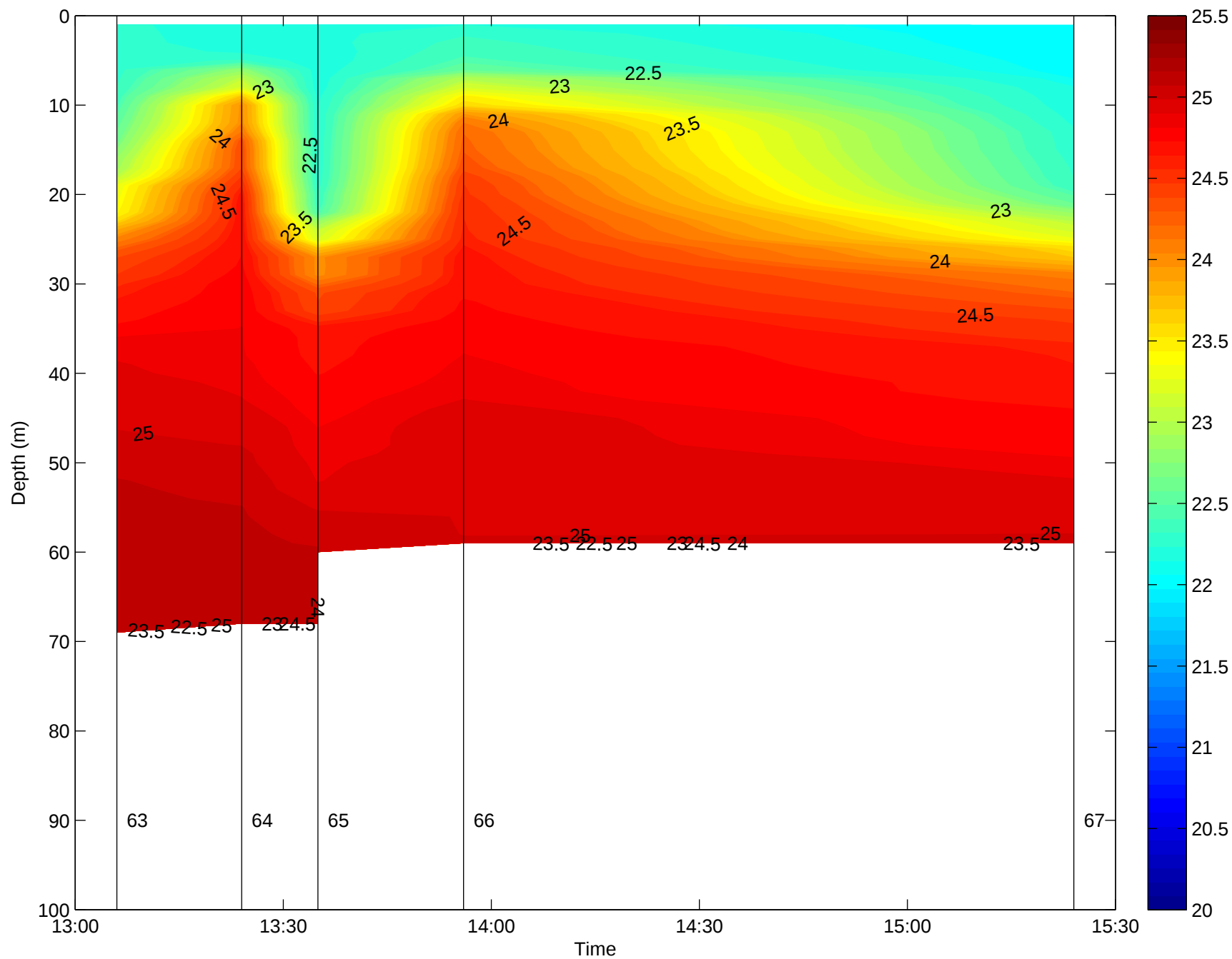
Sigma Theta, Argo Maine Transect 8: 02-Sep-1998 13:06 to 02-Sep-1998 15:24 06:56 after low water to 09:14 after low water
