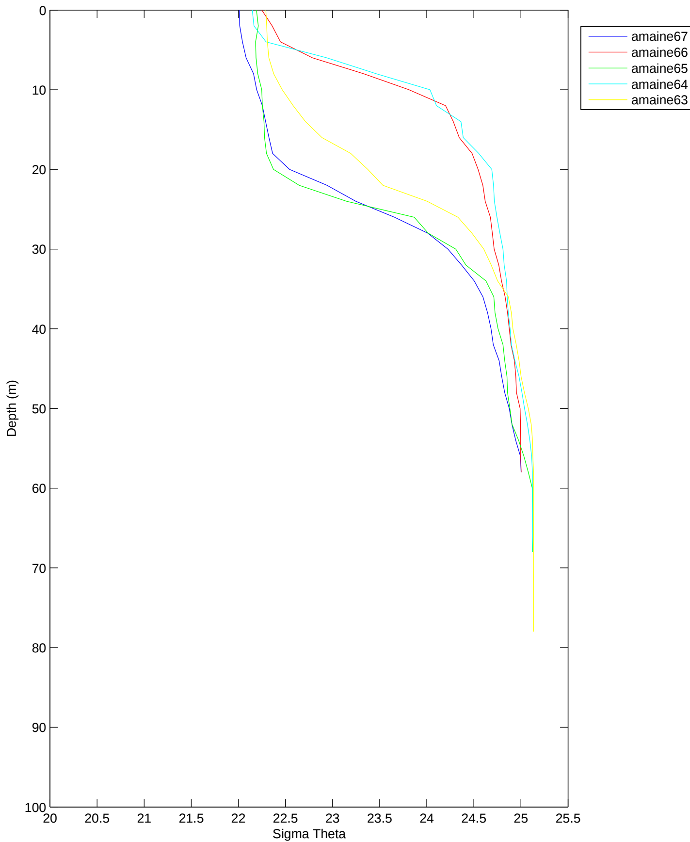
Sigma Theta, Argo Maine Transect 8: 02-Sep-1998 13:06 to 02-Sep-1998 15:24 06:56 after low water to 09:14 after low water
