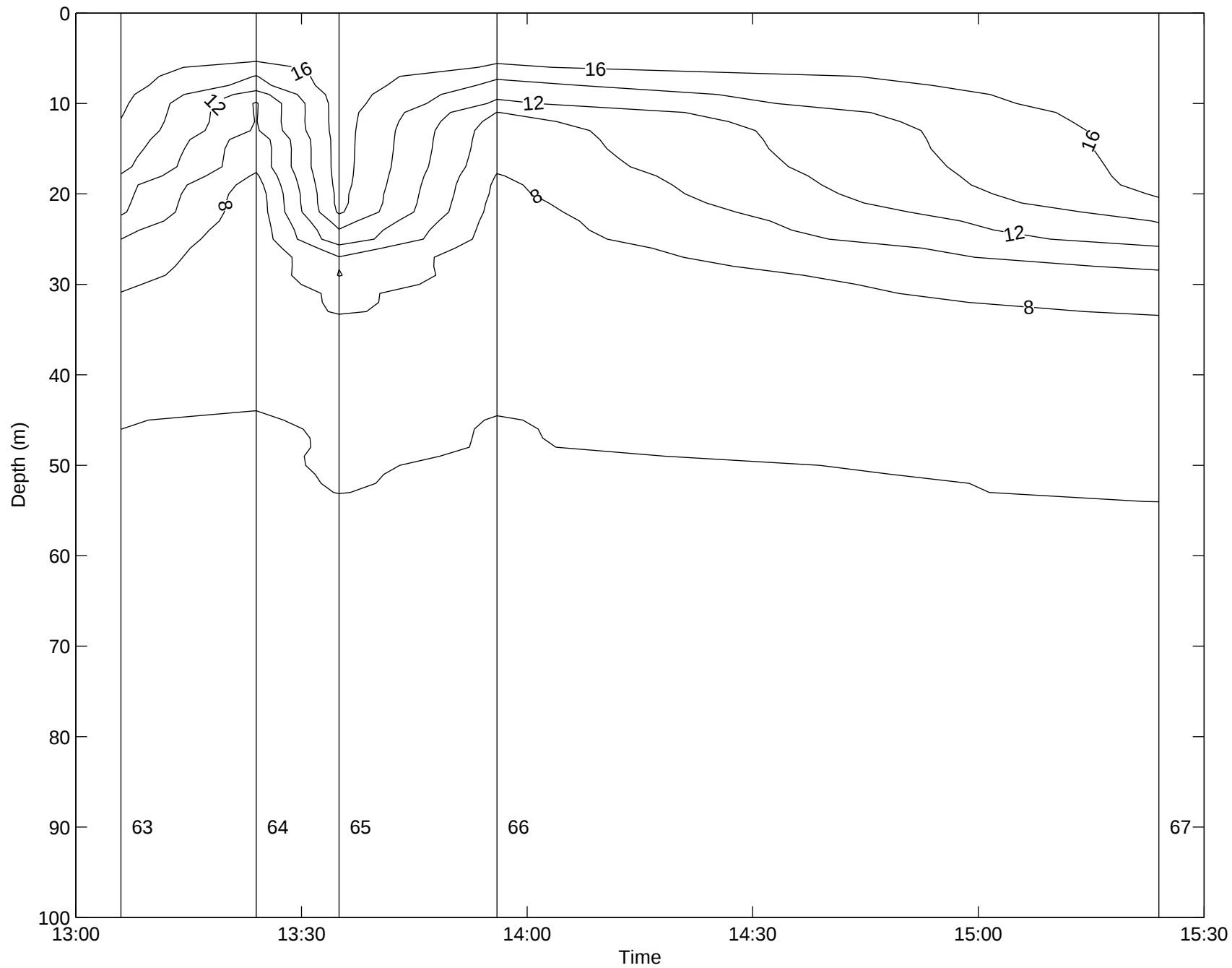
Temperature, Argo Maine Transect 8: 02-Sep-1998 13:06 to 02-Sep-1998 15:24 06:56 after low water to 09:14 after low water
