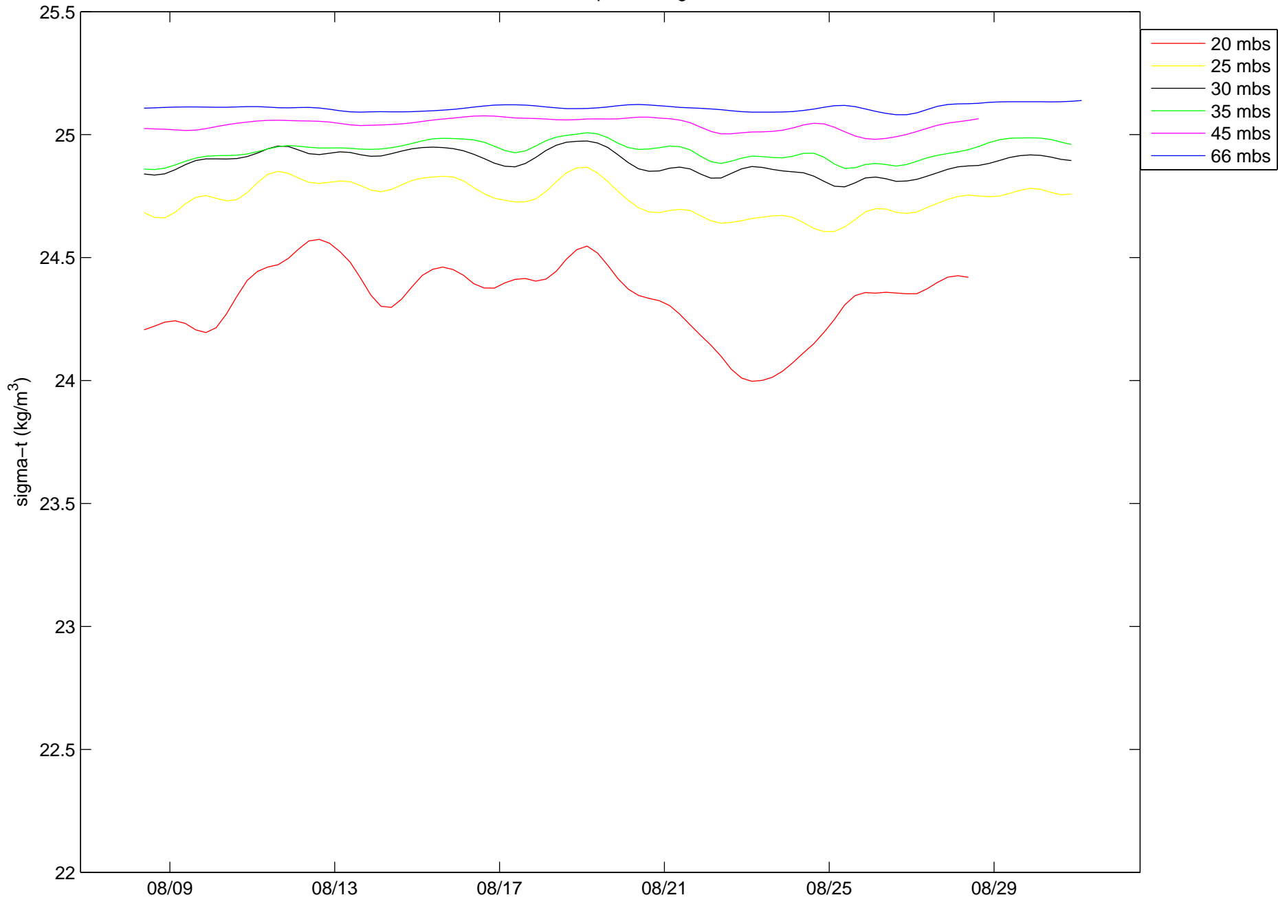
Site B, Low-passed Sigma-t
