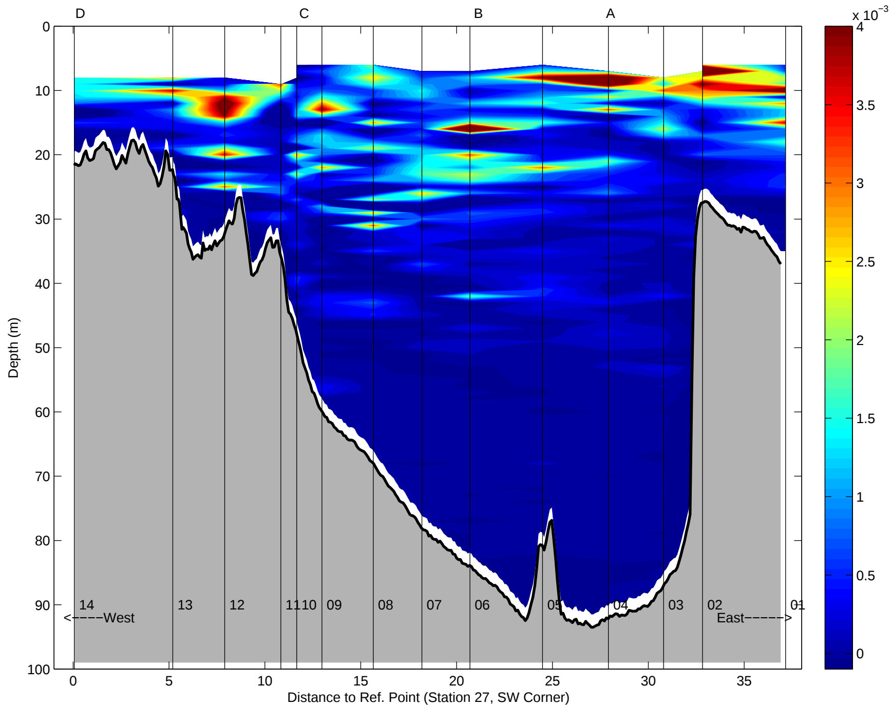
Brunt-Vaisala Frequency, Christopher Andrew Transect 1: 06-Aug-1998 15:28 to 06-Aug-1998 21:41 07:04 after low water to 13:17 after low water
