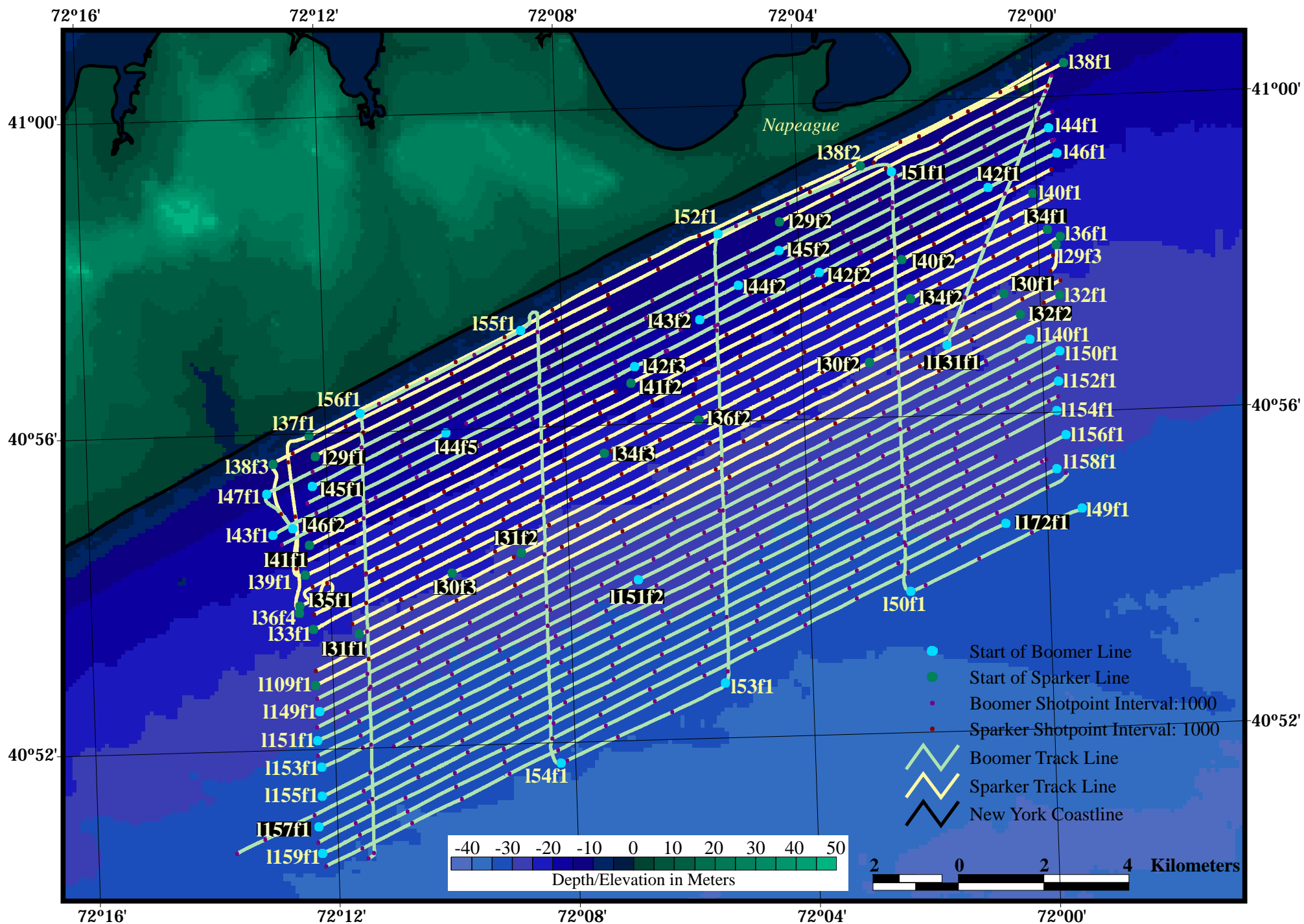
DIAN 97032 Boomer and Sparker Survey Area 4 (Boomer Lines 42-47, 49-56, 131, 140, 149-159, 172; Sparker Lines 29-41, 109)
