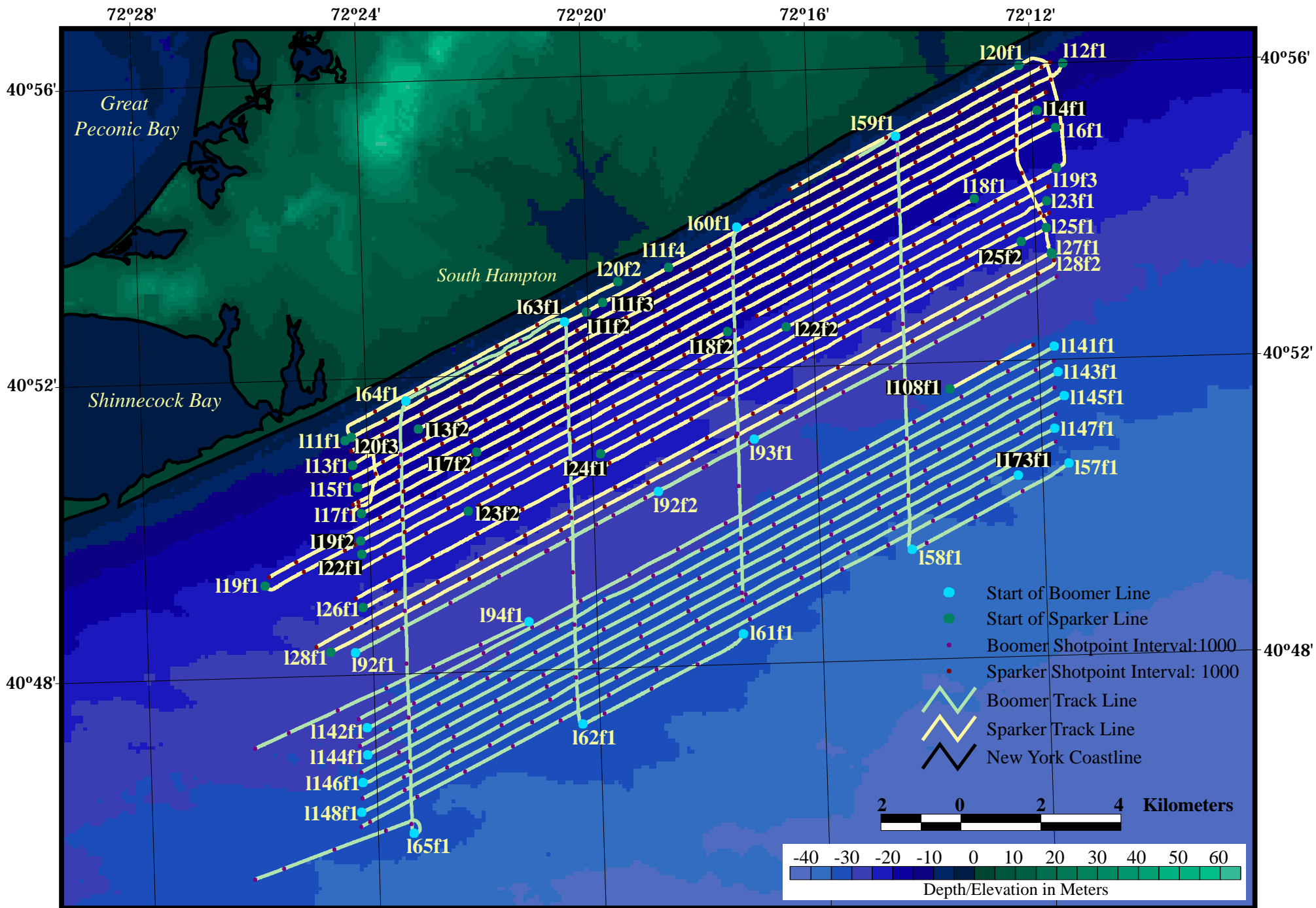
DIAN 97032 Boomer and Sparker Survey Area 3 (Boomer Lines 57-65, 92-94, 141-148, 173; Sparker Lines 11-20, 22-28, 108)
