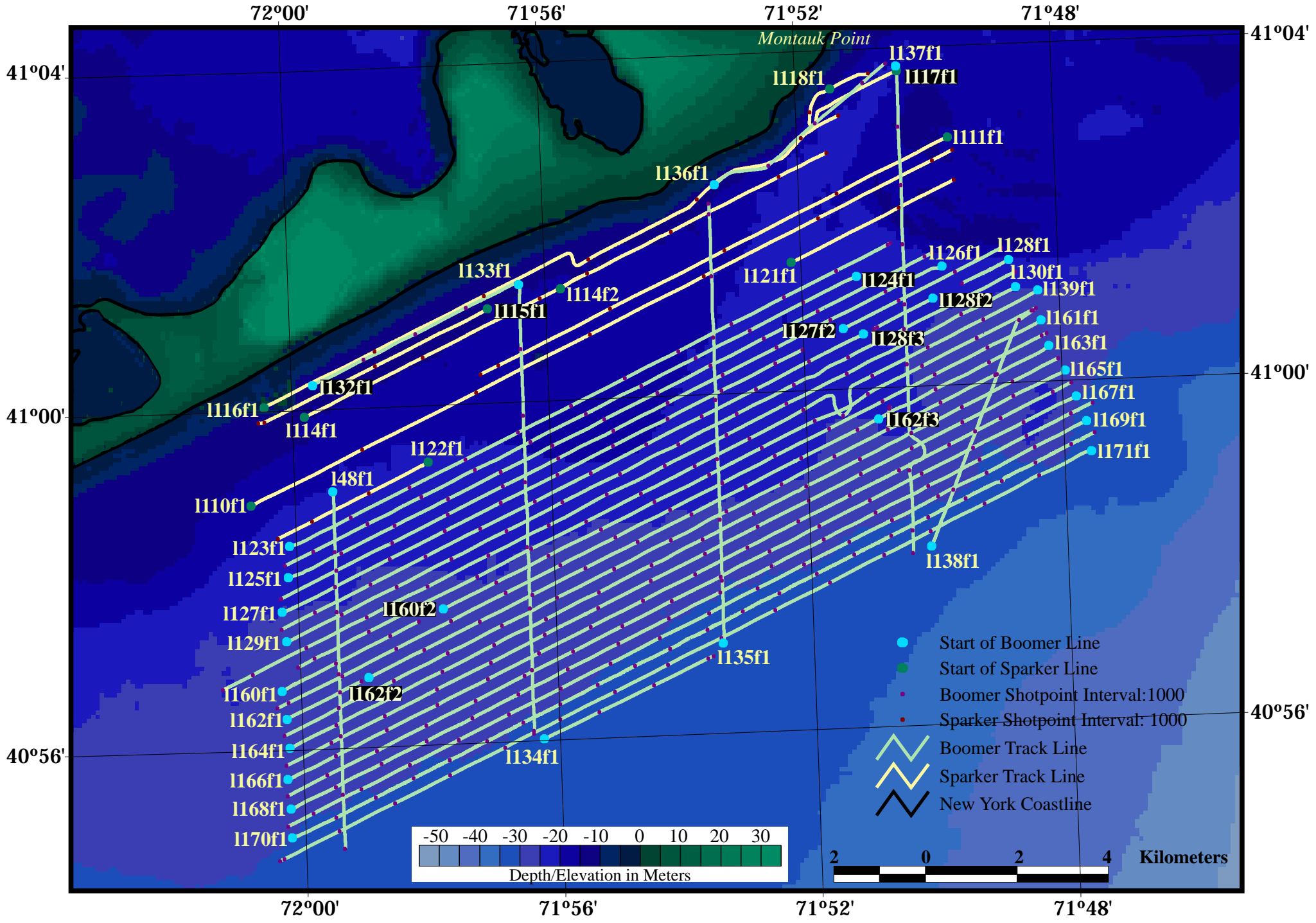
DIAN 97032 Boomer and Sparker Survey Area 5 (Boomer Lines 48, 123-130, 132-139, 160-174; Sparker Lines 110-111, 114-118, 121-122)
