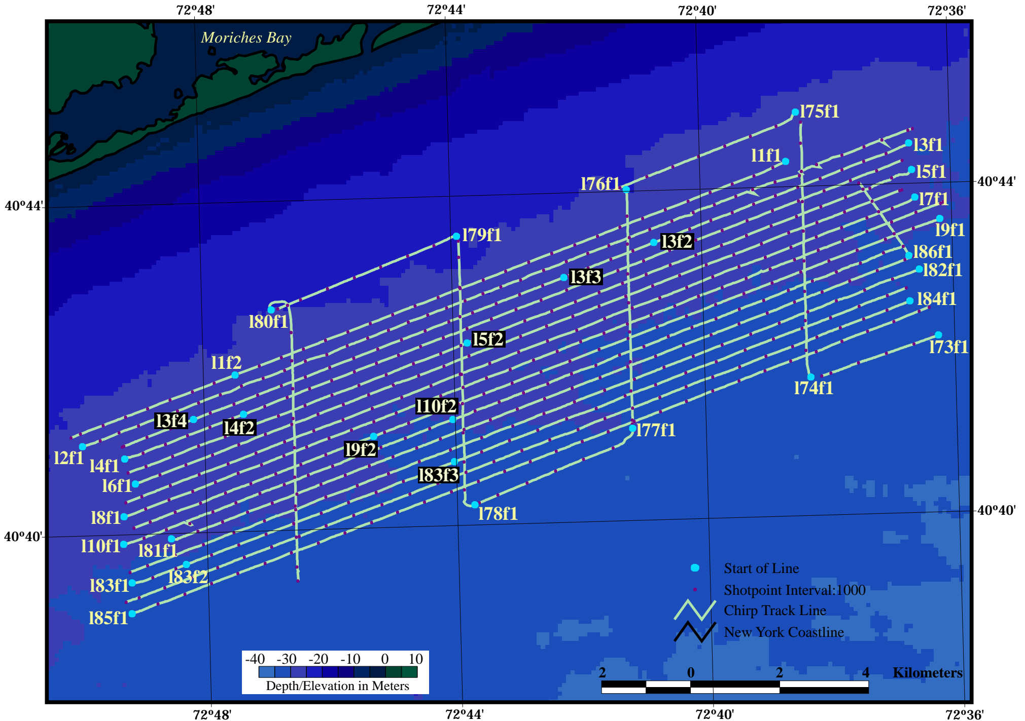
DIAN 97032 Chirp Survey Area 1 (Lines 1-10, 73-86)
