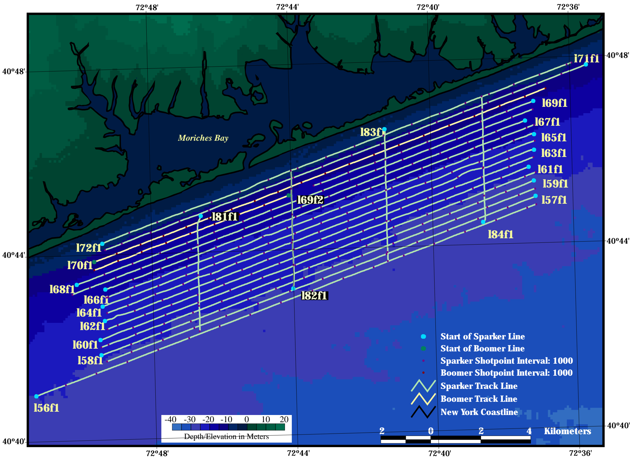
DIAN 97011 Boomer and Sparker Survey Area 4 (Lines 56-72, 81-84)
