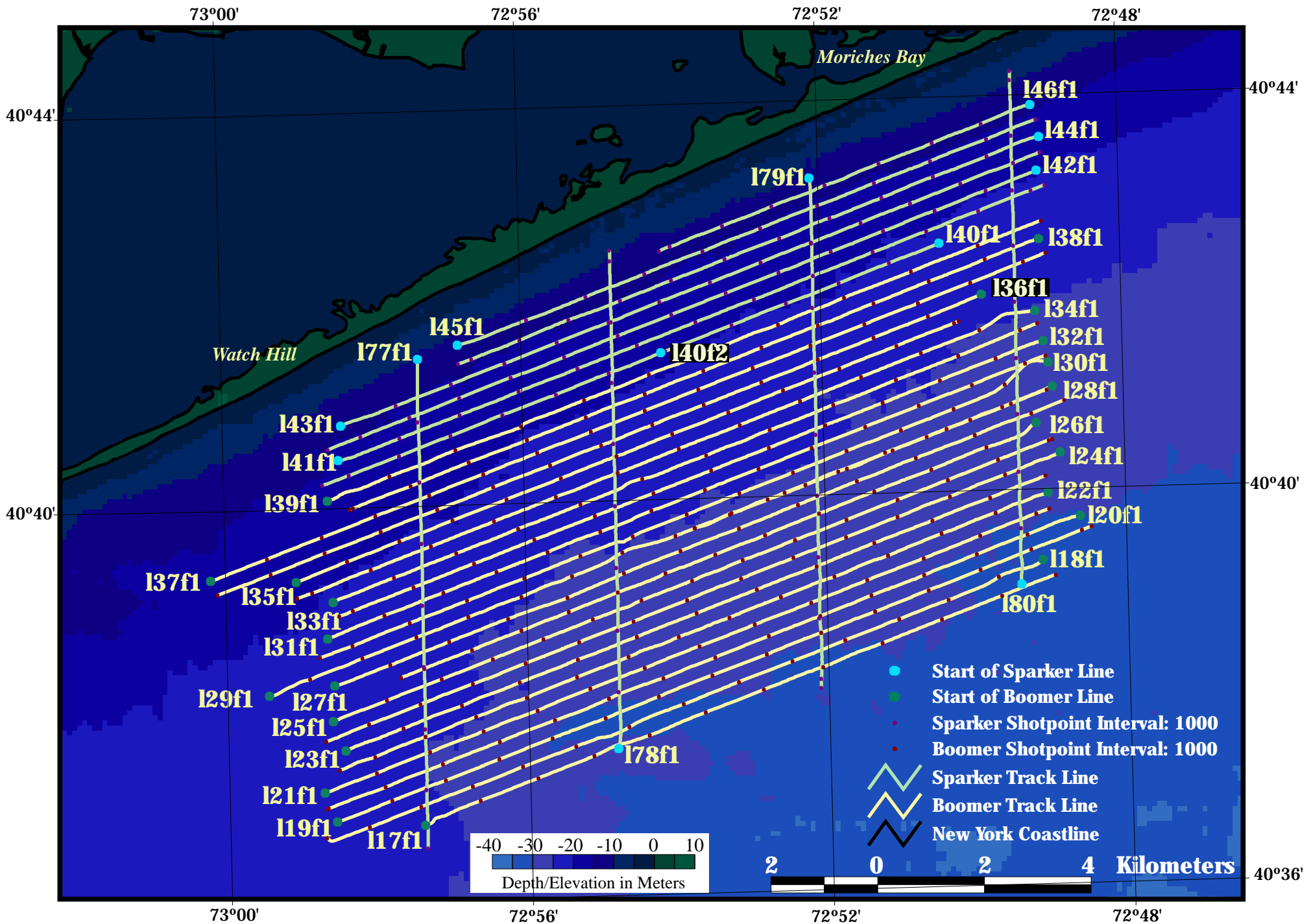
DIAN 97011 Boomer and Sparker Survey Area 3 (Lines 17-46, 77-80)
