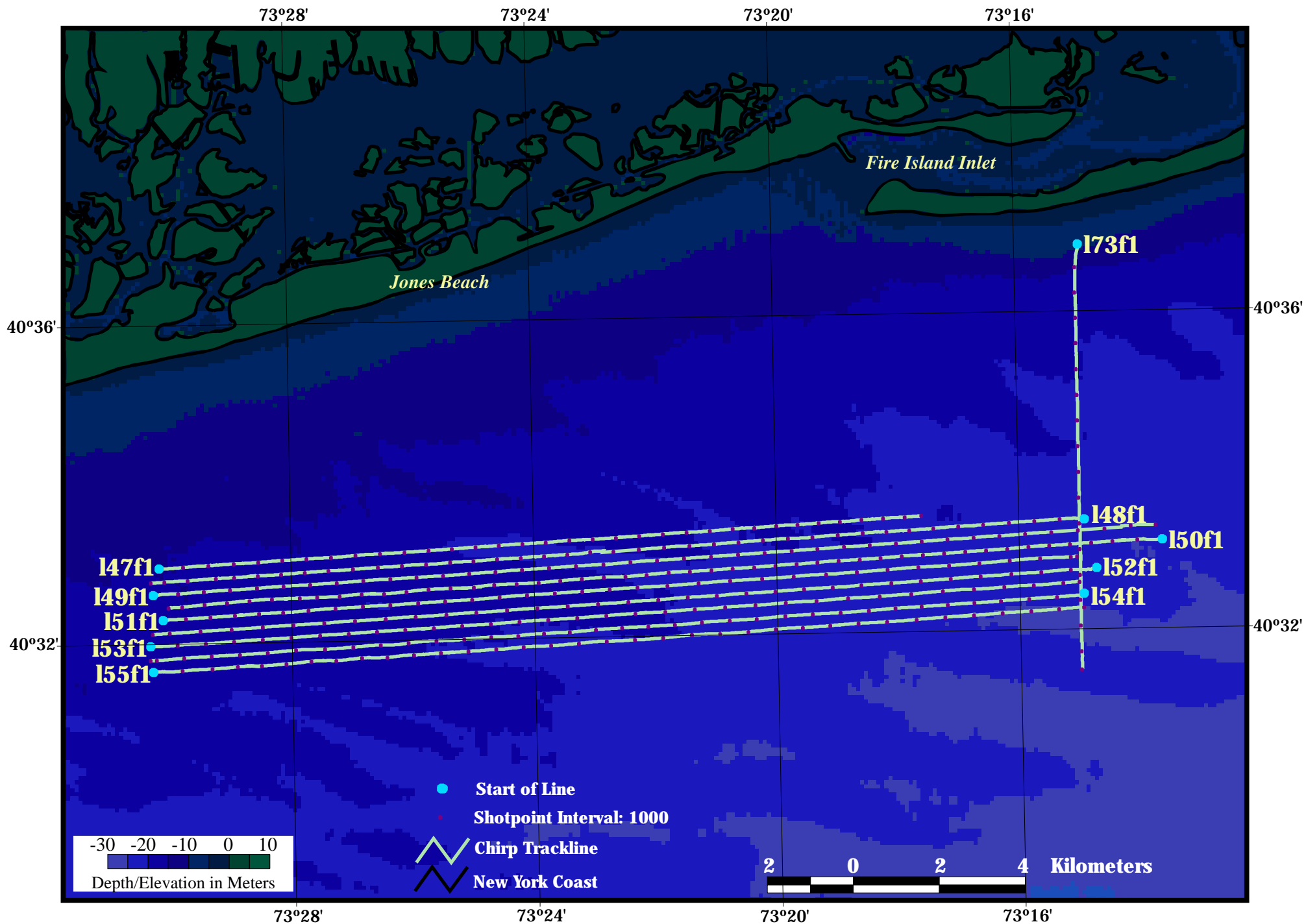
DIAN 97011 Chirp Survey Area 1 (Lines 47-55, 73)
