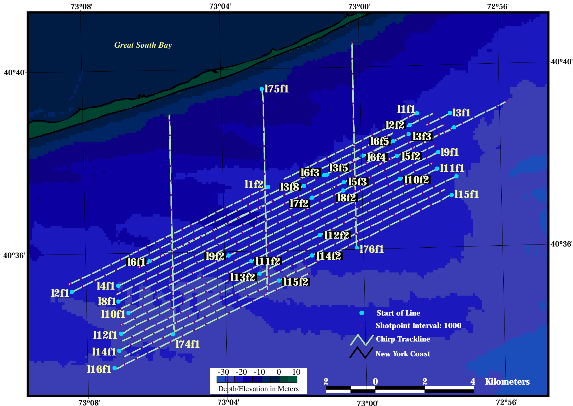
DIAN 97011 Chirp Survey Area 2 (Lines 1-16, 74-76)
